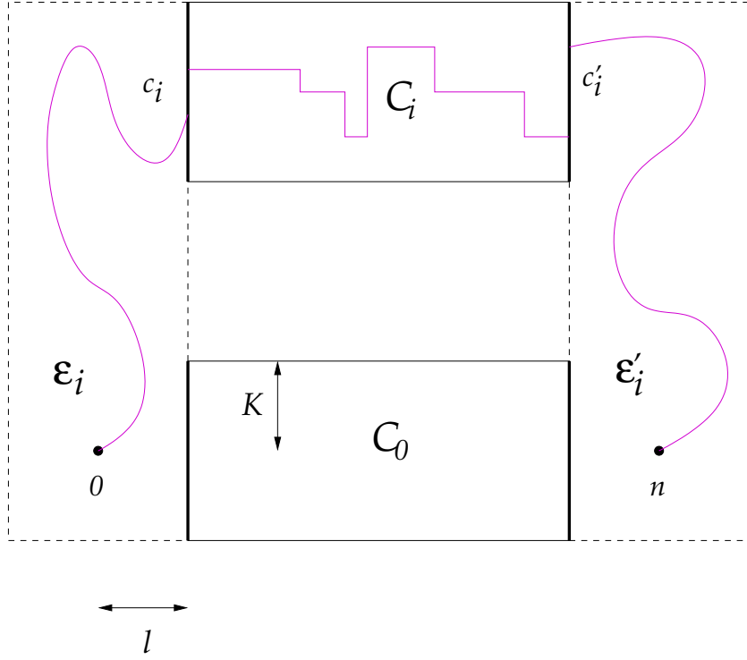
Figure 3: The sketch of an almost optimal path, on the event B_i \cap \{I = i\} .
