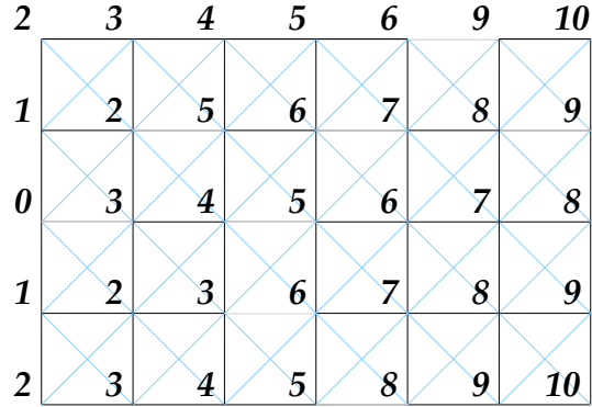
Figure 1: A configuration of percolation in \mathbb{Z}_K for K = 2 , with eight closed edges and the associated distances \mathbf{D}^{K,d} .
