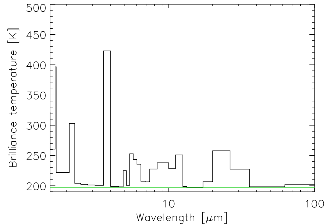
Figure 9. Brightness temperature of the thermal emission of a Venus-like atmosphere.
