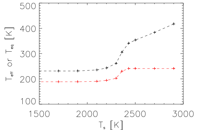
Figure 1. T_{\text{eff}} (black line) and T_{\text{eq}} (red line) versus T_s with P_n = 100 bars and P_v = 300 bars.
