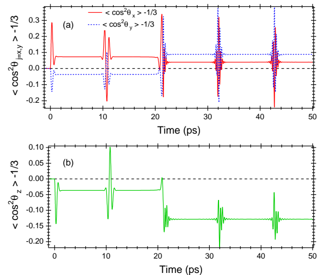
FIG. 3: (Color online) Evolution at T = 100 K of the expectation values (a) \langle \cos^2 \theta_x \rangle (red line), \langle \cos^2 \theta_y \rangle (dotted blue line), and (b) \langle \cos^2 \theta_z \rangle (green line) for the CO 2 molecule exposed to the peak intensities I_y = 120 TW/cm 2 and I_x = I_y/2.2 .
