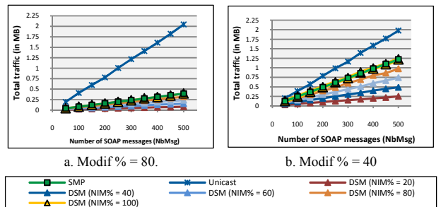
Fig. 10. Network traffic variation, w.r.t. the total number of SOAP messages to be multicast, NbMsg .
