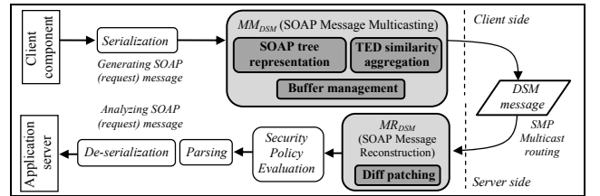
Fig. 2. Outline of our approach 2 .
