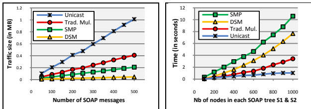
Fig. 11. Network traffic, with NIM % =20 & Modif % =10.
