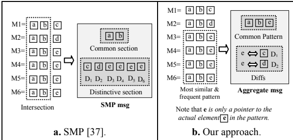
Fig. 1. Motivating example to SOAP message aggregation.
