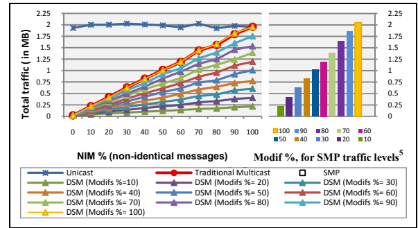
Fig. 9. Variation of total network traffic w.r.t. the amount of modifications between messages, for a total of NbM=500 SOAP messages.
