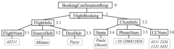
Fig. 5. Sample SOAP message tree representation.
