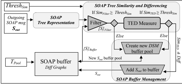
Fig. 3. Simplified activity diagram describing our SOAP message multicasting module, MM_{DSM} .
