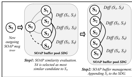
Fig. 8. An Example of SOAP buffer management.
