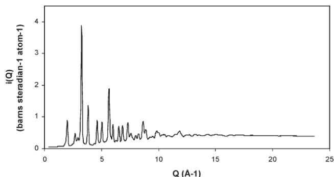
Figure 2. R-U 4 O 9 neutron diffraction pattern corrected from air and sample holder diffusion.
