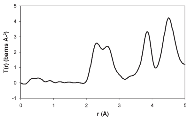
Figure 4. Zoom from 0 to 7 Å of the calculated R-U 4 O 9 T(r) (see the text for details).
