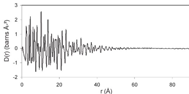
Figure 3. R-U 4 O 9 D(r) obtained by Fourier transformation (see the text for details).
