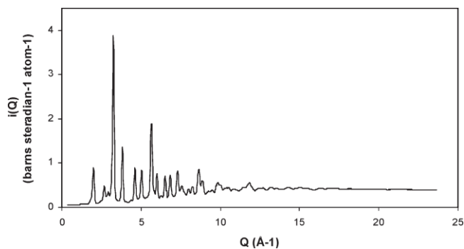
Figure 2. R-U 4 O 9 neutron diffraction pattern corrected from air and sample holder diffusion.
