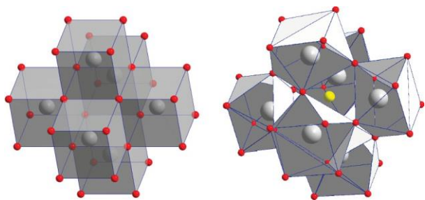
Figure 1. Comparison between the UO 2 lattice (left part) and a cuboctahedron in the B-U 4 O 9 lattice (right part). Uranium atoms are gray, oxygen atoms are red, and the oxygen atom at the center of the cuboctahedron is yellow.
