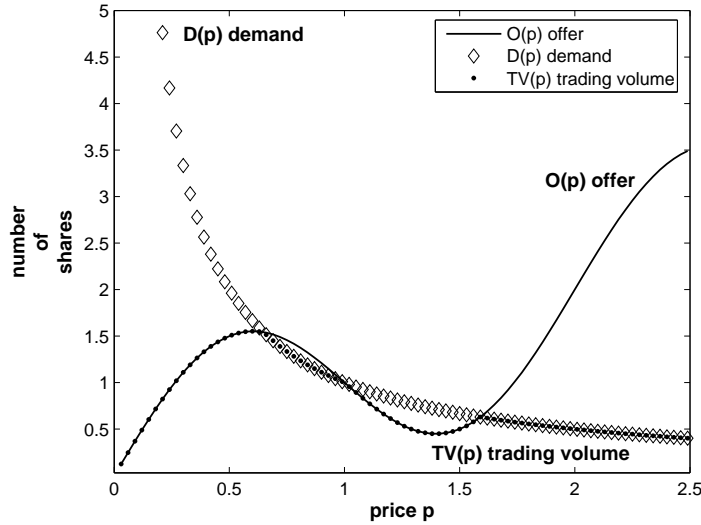
Figure 1: An illustration of Remark 3. Here V = 1 , O(p) = p + \sin(\pi p) and D(p) = 1/p but O(p) is not monotonic. Several prices exist that clear the market. The first price, situated at about p = 0.684 , maximizes the trading volume among the points that clear the market (with value around 1.541) but it does not maximize the trading volume TV(p) whose maximum value is around 1.551.
