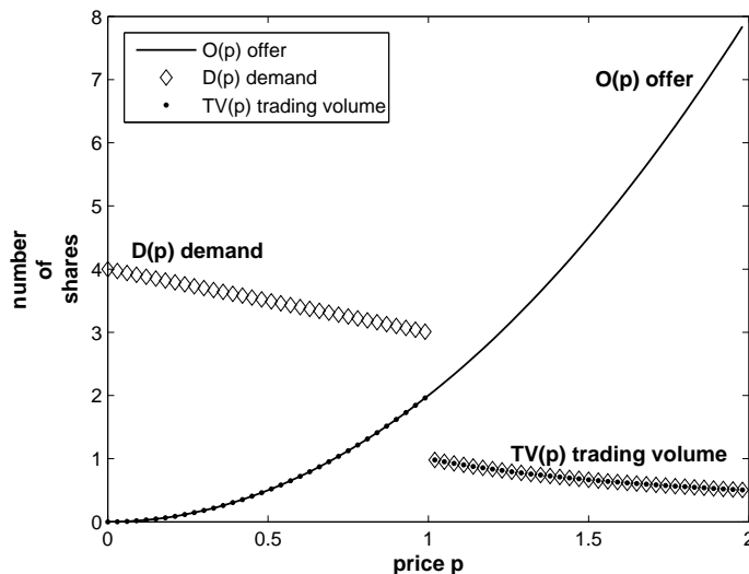
Figure 2: An illustration of the Remark 4: offer and demand functions are discontinuous: no price exists that clears the market; the maximum trading volume is not attained by any price.
