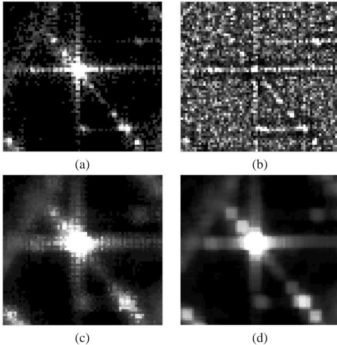
Fig. 3. Toulouse, RAMSES POLSAR data, X-band, 50 \times 50 pixels, zoom image: (a) FP-PWF texture, (b) SCM-PWF normalized texture, (c) span estimated using \widehat{\sigma}_0 from Eq. 9 and (d) SCM-MPWF span.
