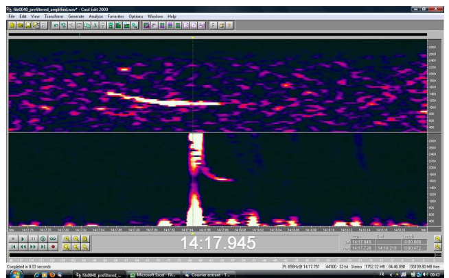
Figure 16 – ELF tweek associated to a VHF meteor ping.
