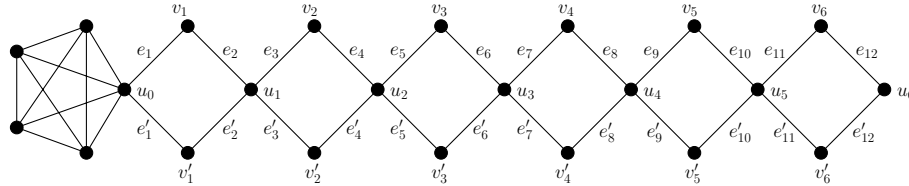
Fig. 3 The graph G with n_C = 6 and n_K = 4 .
