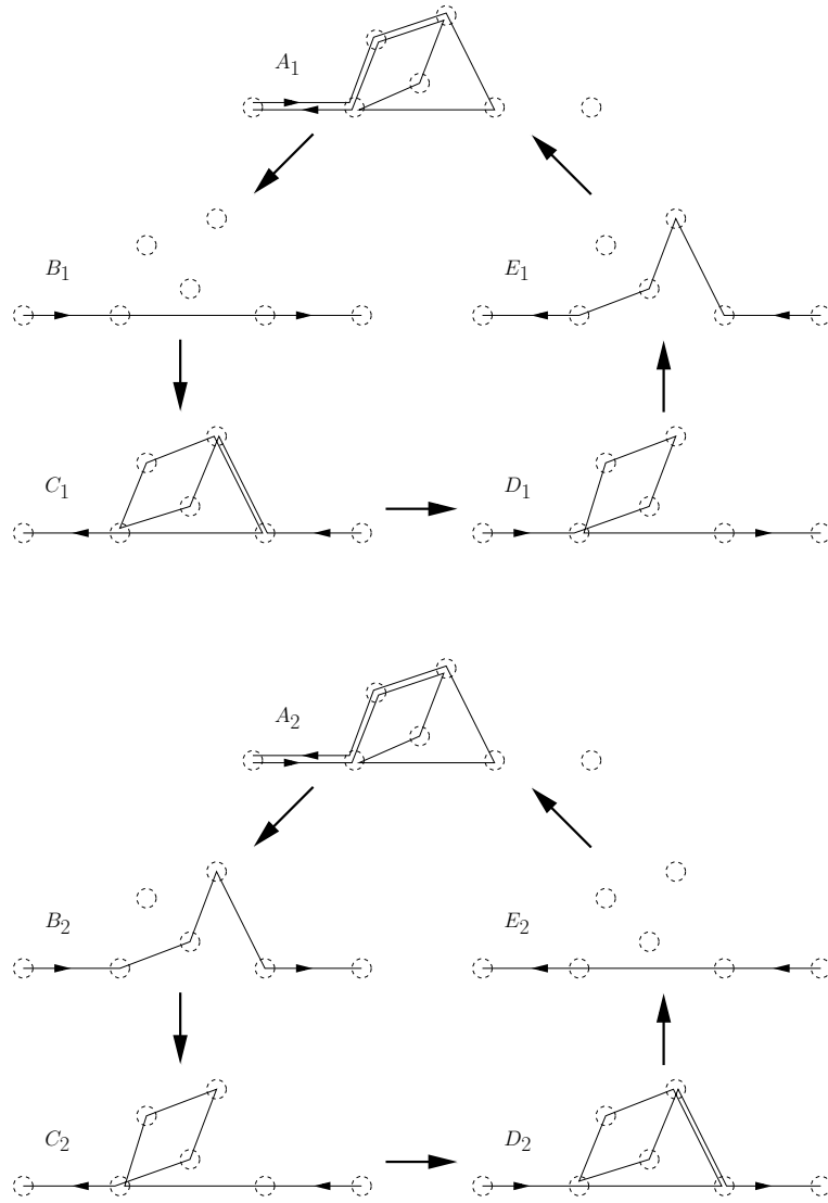
Fig. 2 The two possible cycles of traversals of a block B .
