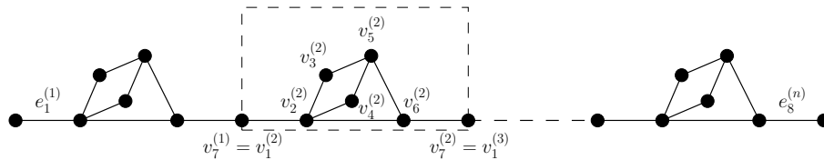
Fig. 1 The graph G_n , a chain of so-called blocks.
