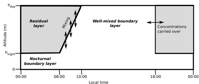
Fig. 5. Conceptual sketch of the two box model.
