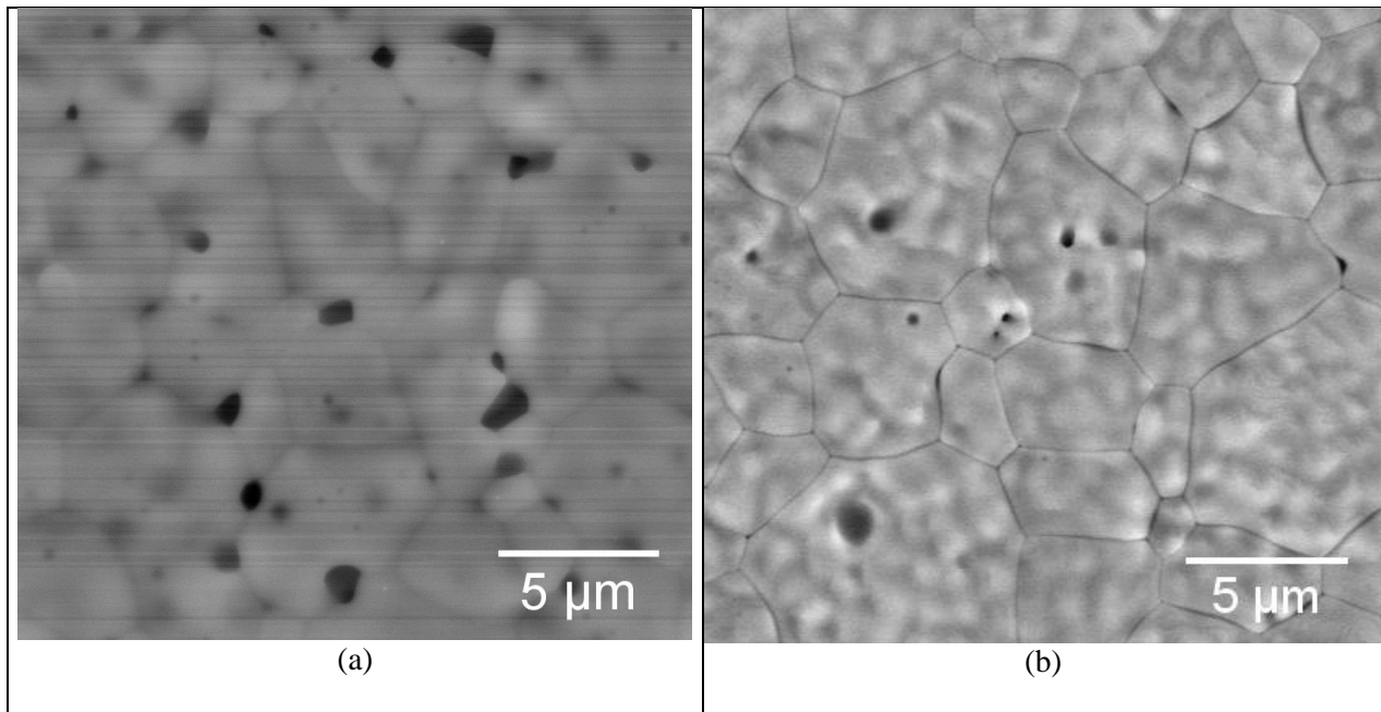
Figure 2 – (a) Typical HT-ESEM image recorded at T=1400^{\circ}\text{C} , after 2.5 hours heat treatment of a \text{CeO}_2 sample. (b) Typical image recorded for a \text{CeO}_2 sample heated for 2.5 hours at T=1400^{\circ}\text{C} in a furnace then cooling at room temperature.
