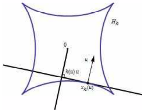
Figure 3. A hedgehog with a C^2 -support function
