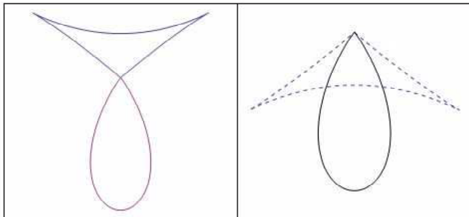
Figure 7. Generatrices of revolution hedgehogs with the same curvature
