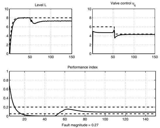
Fig. 7. Medium severity fault effect.
