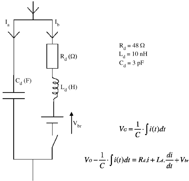
Fig. 7. Electrical model.
