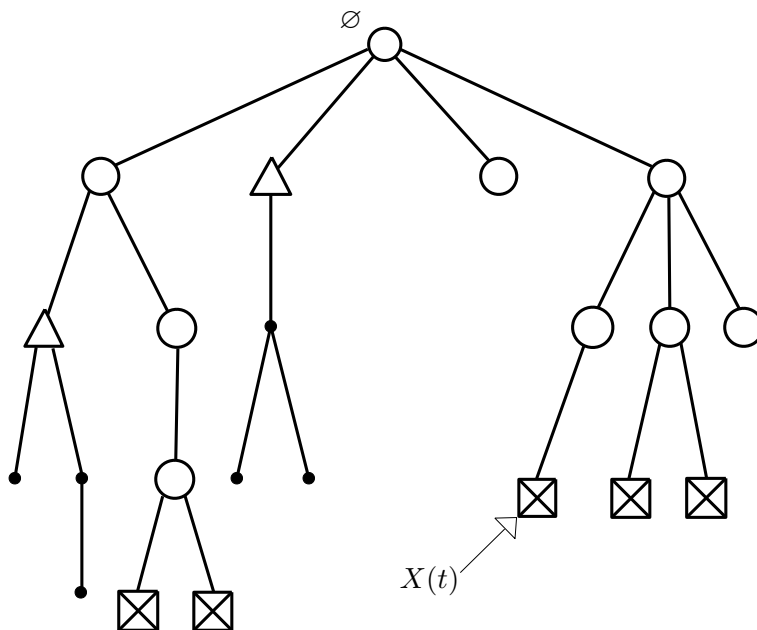
Figure 1. The Galton-Watson tree is represented up to the 4th generation.
