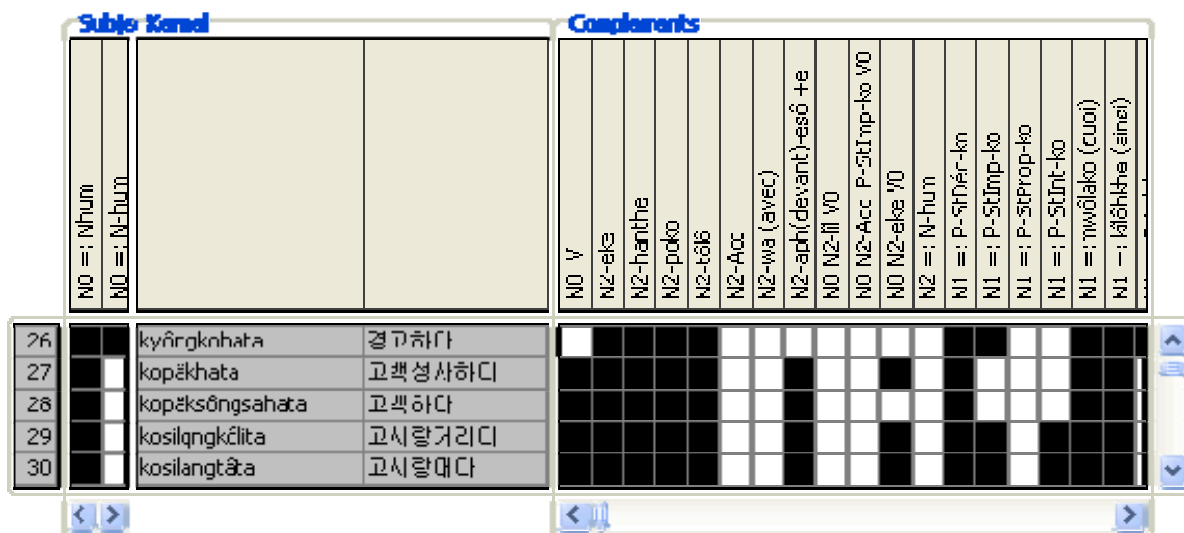
Figure 4 : Fragment of LGT for Korean verbs. A transcription to Latin characters is given.
