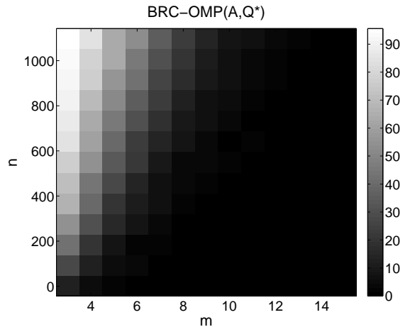
(a) Gaussian dictionaries
