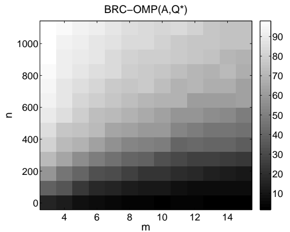
(b) Hybrid dictionaries ( T = 10 )
