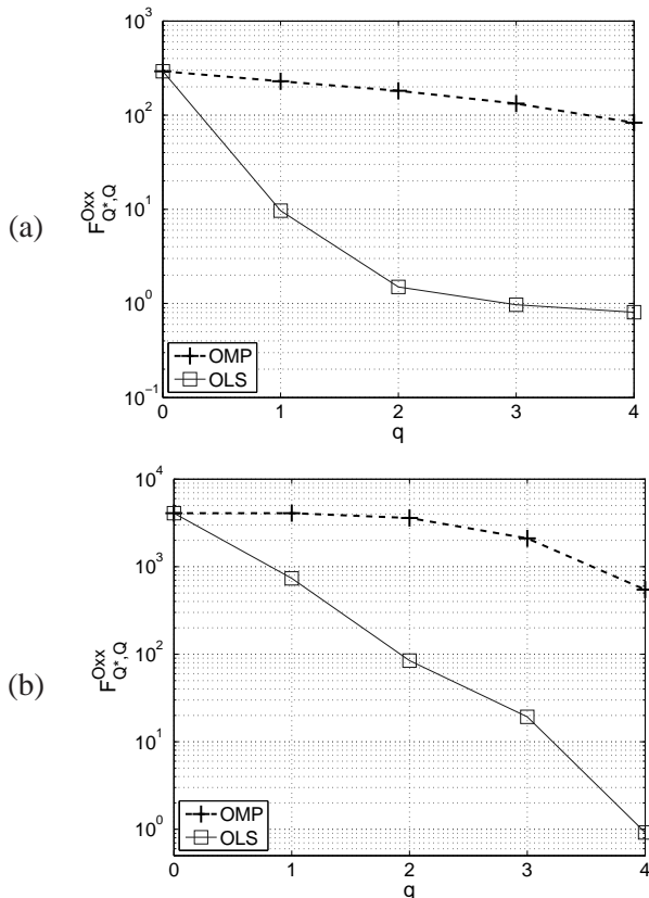
Fig. 4. Curve representing F_{Q^*, Q}^{Oxx} as a function of q = \text{Card}[Q] for the Gaussian deconvolution problem. Q^* is fixed and Q \subseteq Q^* is gradually growing. Q^* and Q are formed of the first k = 5 and the first q atoms, respectively with q < k . (a) The Gaussian impulse response is of width \sigma = 50 and the dictionary is of size 3000 \times 2710 . (b) \sigma is set to 10, and the dictionary is of size 1000 \times 4940 .
