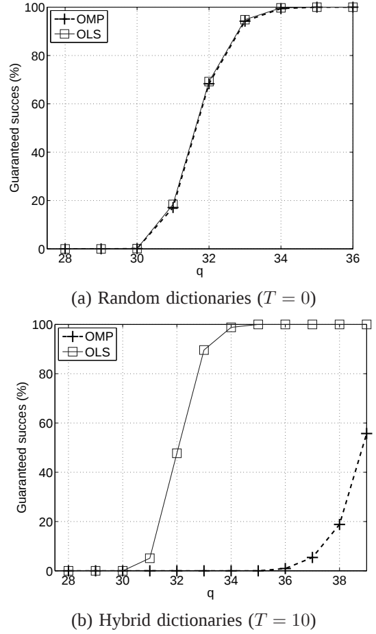
Fig. 2. Phase transition curves: for each q < k , we count the rate of trials where \text{ERC-Oxx}(\mathbf{A}, \mathcal{Q}^*, \mathcal{Q}) is true, with \text{Card}[\mathcal{Q}] = q . The dictionaries are of size 200 \times 600 , k is set to 40 and 1,000 Monte Carlo trials are performed. (a) Randomly Gaussian dictionaries; (b) Hybrid dictionaries with T = 10 .
