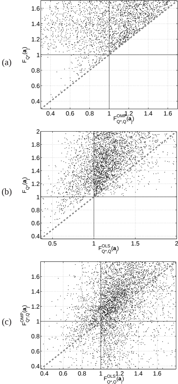
Fig. 1. Comparison of the OMP and OLS exact recovery conditions. We draw 10,000 Gaussian dictionaries of size 100 \times 11 and set k = 10 so that there is only one wrong atom \mathbf{a}_j . \mathcal{Q} is always set to the first atom ( \text{Card}[\mathcal{Q}] = 1 ). Plot of (a) F_{\mathcal{Q}^*}(\mathbf{a}_j) vs F_{\mathcal{Q}^*,\mathcal{Q}}^{\text{OMP}}(\mathbf{a}_j) ; (b) F_{\mathcal{Q}^*}(\mathbf{a}_j) vs F_{\mathcal{Q}^*,\mathcal{Q}}^{\text{OLS}}(\mathbf{a}_j) ; (c) F_{\mathcal{Q}^*,\mathcal{Q}}^{\text{OMP}}(\mathbf{a}_j) vs F_{\mathcal{Q}^*,\mathcal{Q}}^{\text{OLS}}(\mathbf{a}_j) . For the last subfigure, we keep the trials for which F_{\mathcal{Q}^*}(\mathbf{a}_j) \geq 1 .
