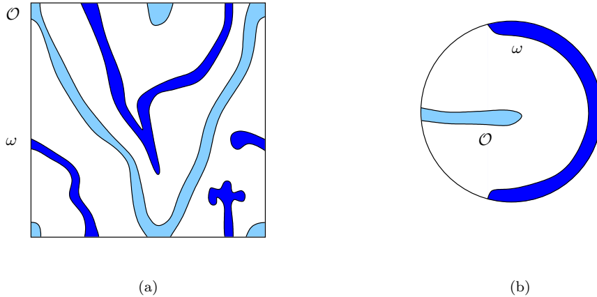
Figure 1: Examples of open sets (\Omega, \omega, \mathcal{O}) such that \omega and \mathcal{O} both satisfy GCC in \Omega , with \omega \cap \mathcal{O} = \emptyset : in the case (a), \Omega is the flat torus (or the square), in the case (b), \Omega is the disk.
