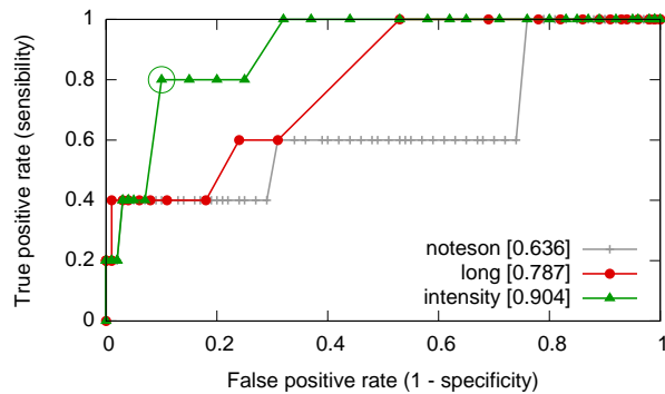
Figure 10. Best ROC Curves, with associated AUC, for retrieving all 5 versions of Christ lag in Todesbanden from BWV 278 in a set of 404 chorales.
