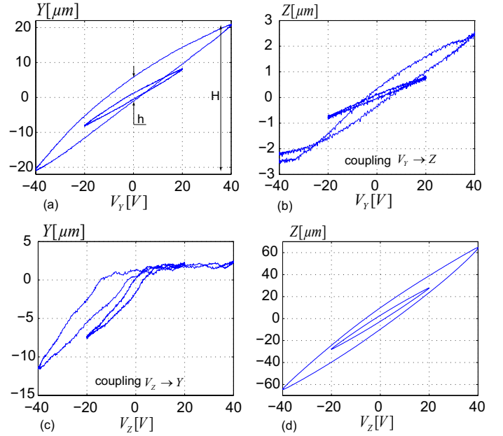
Fig. 5. Hysteresis characteristics of the 2-DOF system piezocantilever.
