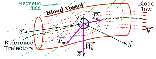
Fig. 3. Forces applied on microrobot navigating in blood vessel.
