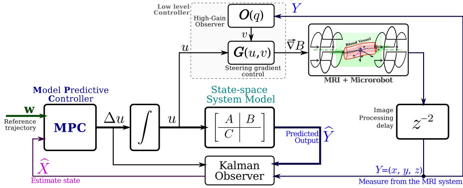
Fig. 4. MRI-based Predictive Control strategy.
