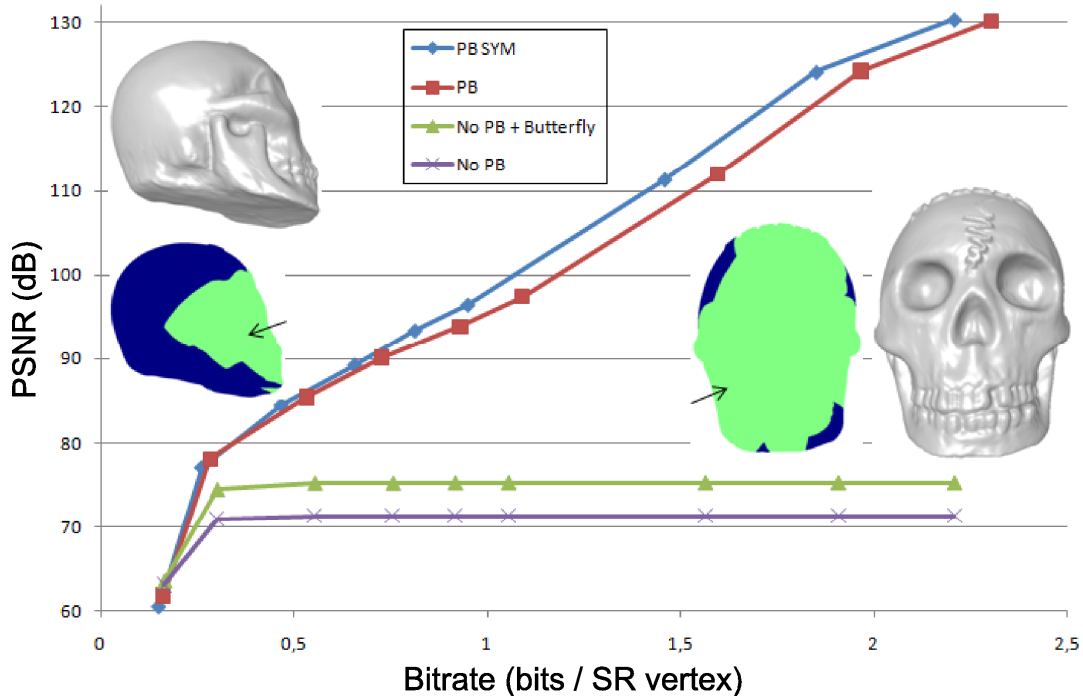
Figure 18: Bitrate- PSNR curves for the non-smooth region of the segmented Skull model, where the Butterfly prediction is used (without any wavelets) in the smooth region. The bitrate (reported in bits/SR vertex) corresponds to the bit allocation after quantization, with respect to the number of vertices in the SR non-smooth patch.
