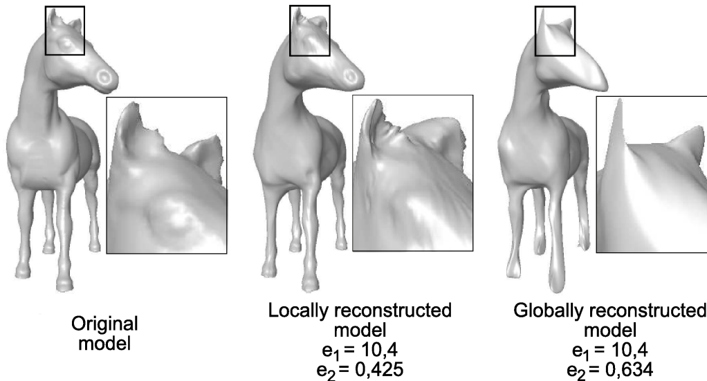
Figure 20: Comparison of two different reconstructions of the Horse Normal model based on a local (middle) and a global (right) wavelet decomposition. The reconstruction presented in the middle, was produced with our framework on the segmented Horse model. Here the Butterfly prediction is followed by a wavelet addition only in non-smooth regions. We have reported the corresponding distortion errors e_1 and e_2 , which correspond respectively to the MSE (in units of 10^{-4} ) and to Lavoué et al. 's MSDM metric [37].
