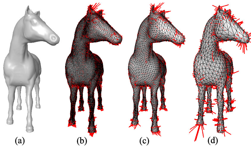
Figure 5: (a) Original Normal Horse model; (b-d) Wavelet coefficients represented as 3D vectors (in red) linked to the edges of the first three decompositions (multiplication factor used to emphasize them: 10).
