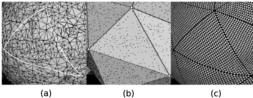
Figure 3: Overview of a semi-regular remeshing. Each vertex in the area bounded by white curves (a) is projected in one triangle of the base complex (black dots on (b)). The SR mesh (c) is then obtained by iterative subdivision and by mapping the new vertices onto the surface using the parameterization. Image of [9].
