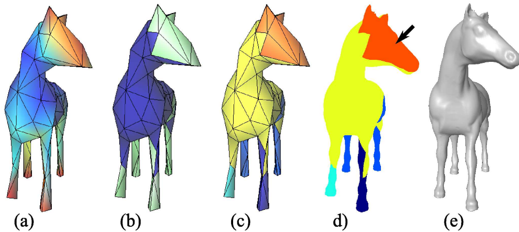
Figure 10: Illustration of the different steps involved in our classification and segmentation processes, on the 5 th level of the Normal Horse model. (a) Averaging of the wavelet norms in the 5 th level followed by (b) the K-Mean classification and (c) segmentation in 5 regions; (d) Fine projection of the segmentation on the SR original model whose features can be better appreciated with a Phong shading (e).
