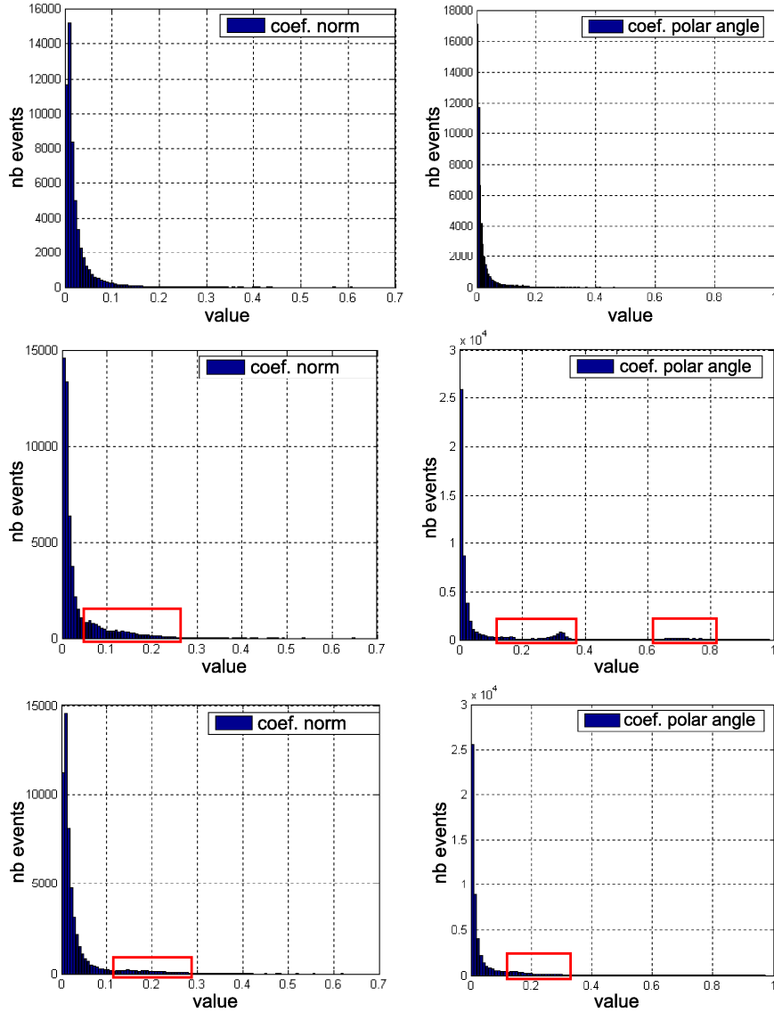
Figure 13: Amplitude (left) and polar angle (right) distributions in every resolution level of the Venus Normal segmented model (right segmentation of Fig. 11 considered). The red boxes highlight the differences noticed in the two "PB" distributions (middle: classical rule - bottom: our new rule), in comparison with the distributions for which the classical Butterfly stencil was used, without taking into account the patch borders (top).
