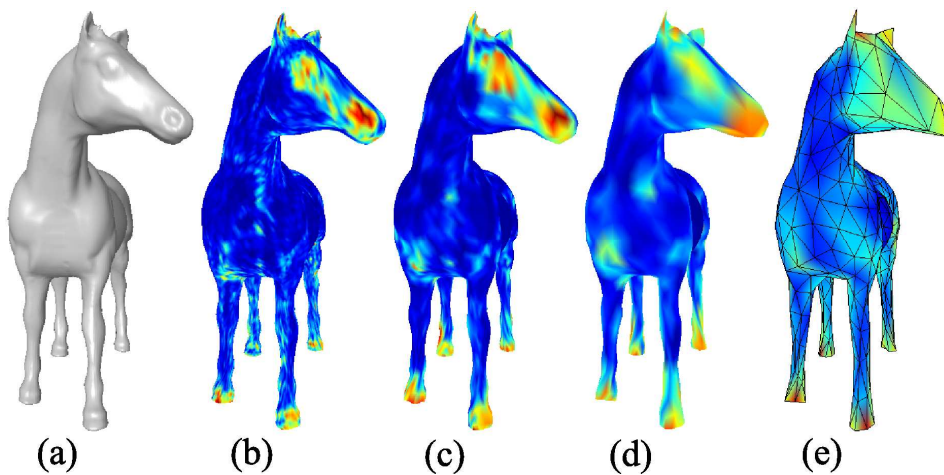
Figure 7: Gaussian normalized distributions of the wavelet coefficient norm, on the first four resolution levels of the Normal Horse model.
