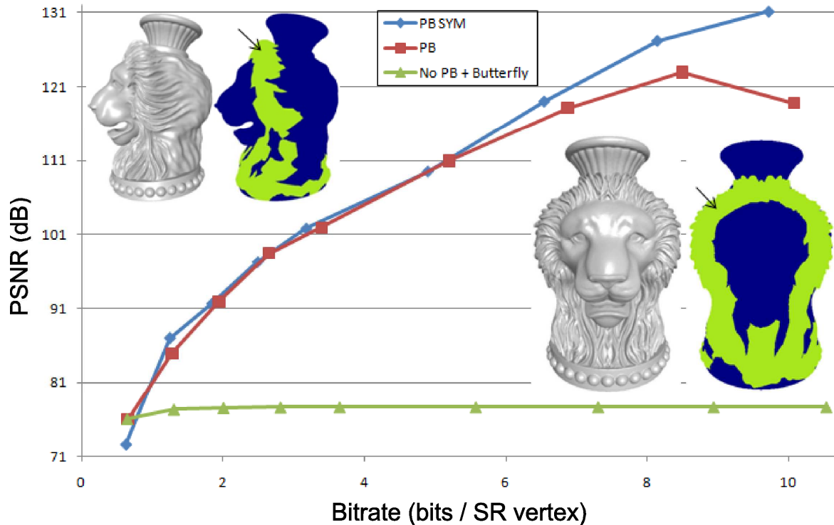
Figure 19: Bitrate- PSNR curves for the non-smooth region of the segmented Lion Head model, where the Butterfly prediction is used (without any wavelets) in the smooth region. The bitrate (reported in bits/SR vertex) corresponds to the bit allocation after quantization, with respect to the number of vertices in the SR non-smooth patch.
