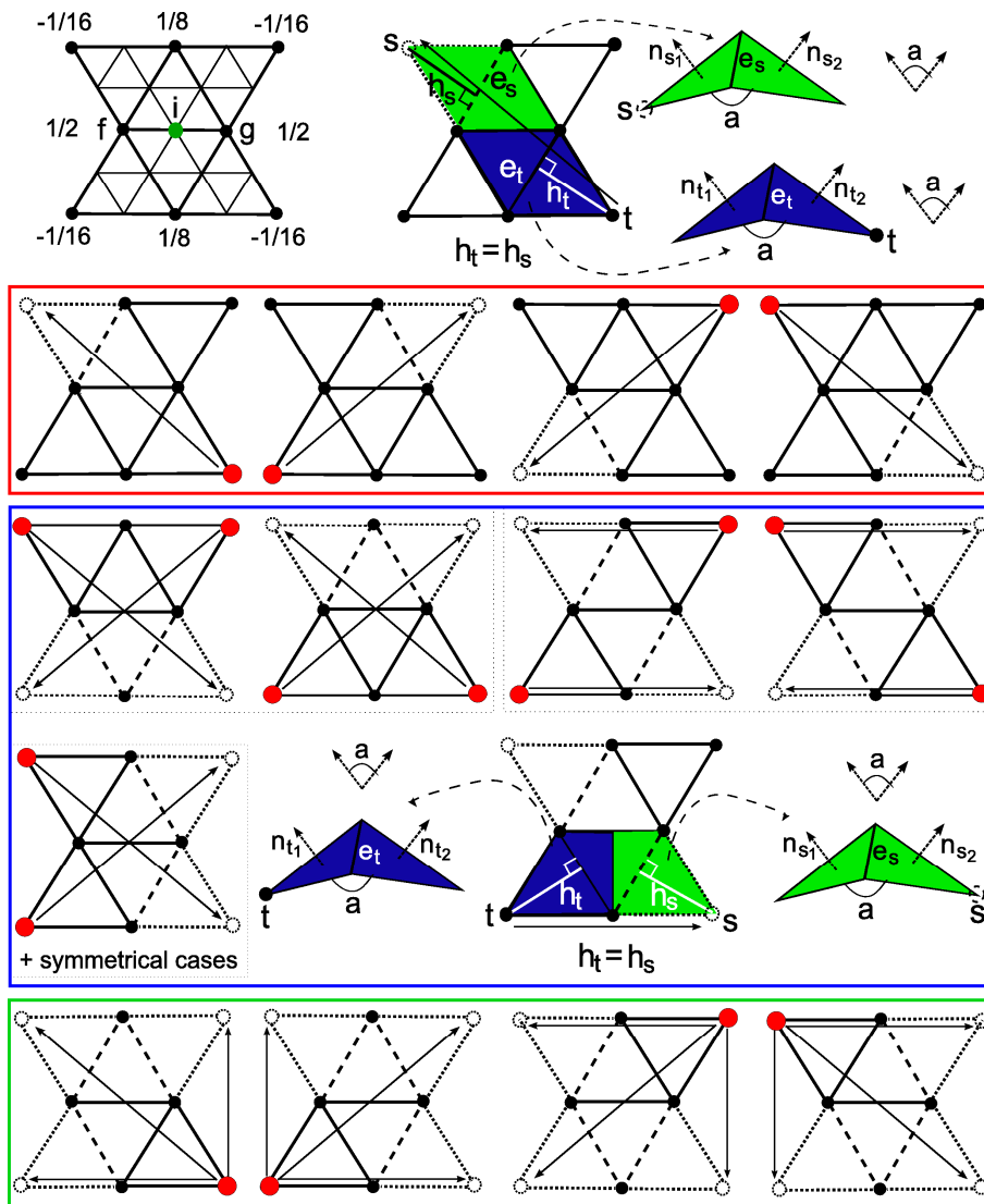
Figure 15: Definition of our new scheme, used when some of the coarse vertices are missing in the Butterfly stencil, due to patch borders (illustrated with big dashed lines). Top left: classical Butterfly stencil; Top right: method used to recreate the "missing coarse vertices" in the Butterfly stencil. We favor the diagonal symmetry (computed thanks to the red vertices in the
