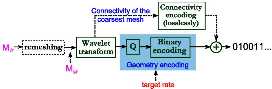
Figure 16: Main steps of a wavelet-based coder for SR meshes. Q stands for the Quantization step. The geometry encoding is generally done under a constraint which can be user-defined or automatic. This parameter can be a file size [5], a rate [8, 33], a reconstruction quality, etc.
