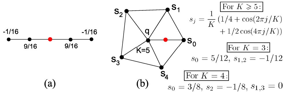
Figure 14: (a) Special Butterfly stencil used to predict the red vertex, situated on the mesh border (for non-closed 3D meshes); (b) Extension of the classical Butterfly stencil for extraordinary vertices (scheme proposed by Zorin et al. [26]).
