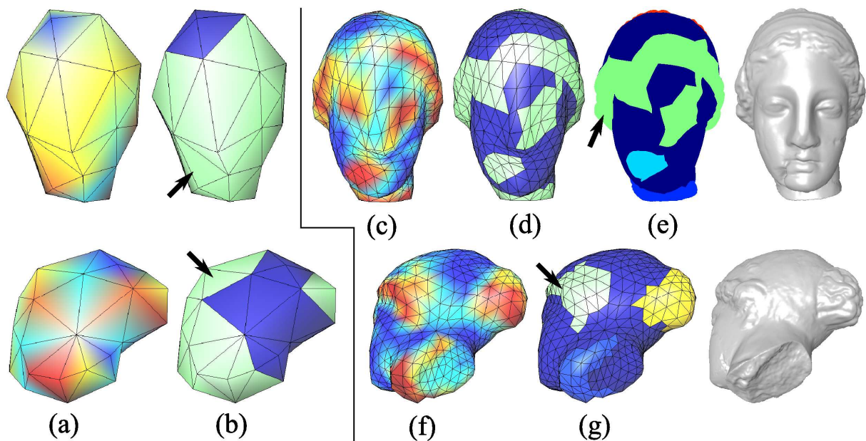
Figure 11: Illustration of the different steps involved in our classification and segmentation processes, on the 6 th (left) and the 4 th (right) levels of the Normal Venus model. (a, c, f) Averaging of the wavelet norms in a coarse level followed by (b, d) the K-Mean classification and (g) segmentation in 6 regions (on the 4 th level). Three regions are obtained in the 6 th decomposition (left). (e) Fine projection of the 4 th level segmentation on the SR original model.
