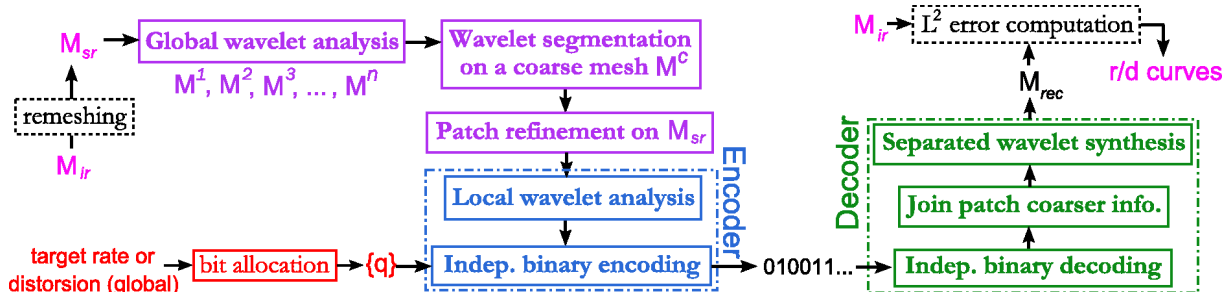
Figure 1: Main features and stages of our framework which aims at locally coding and transmitting a SR mesh M_{sr} (remesh of the original irregular model M_{ir} ). Our framework minimizes the reconstruction error for a given bit budget (target rate), with an error-driven wavelet coefficient quantization ( q ). This allows a flexible reconstruction M_{rec} at the decoder side, where a view-dependent rendering can, for example, be considered. To measure the quality of the reconstructed mesh at a given rate we use rate-distortion ( r/d ) curves (an example is given in Fig. 18 ).
