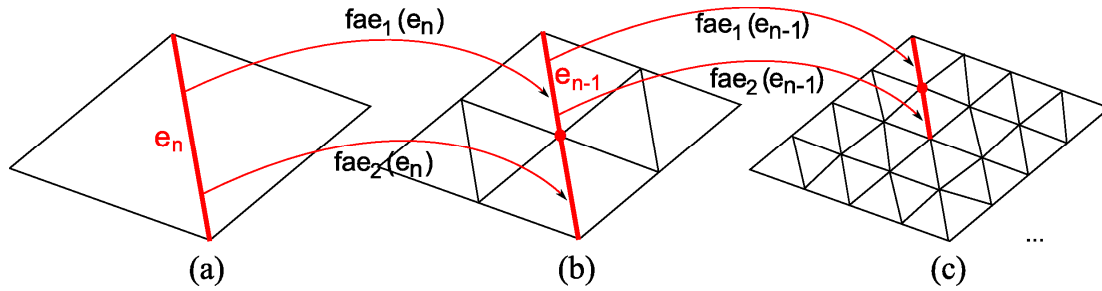
Figure 9: Wavelet "fine averaging association". For an edge e_n in a coarse decomposition, we compute an averaging of its wavelet norm and the norms of its finer associated edges ( fae ) in all the existing resolution levels.
