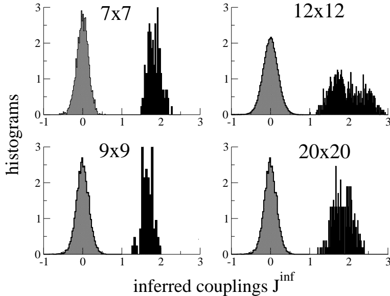
FIG. 24: Histograms of inferred couplings for bidimensional grids of different sizes. Couplings equal to J = 1.778 and 0 in the model are shown in, respectively, black and gray; the integral of each sub-distribution is normalized to one by hand. The values of \Theta^* for each size are shown in Fig. 23.
