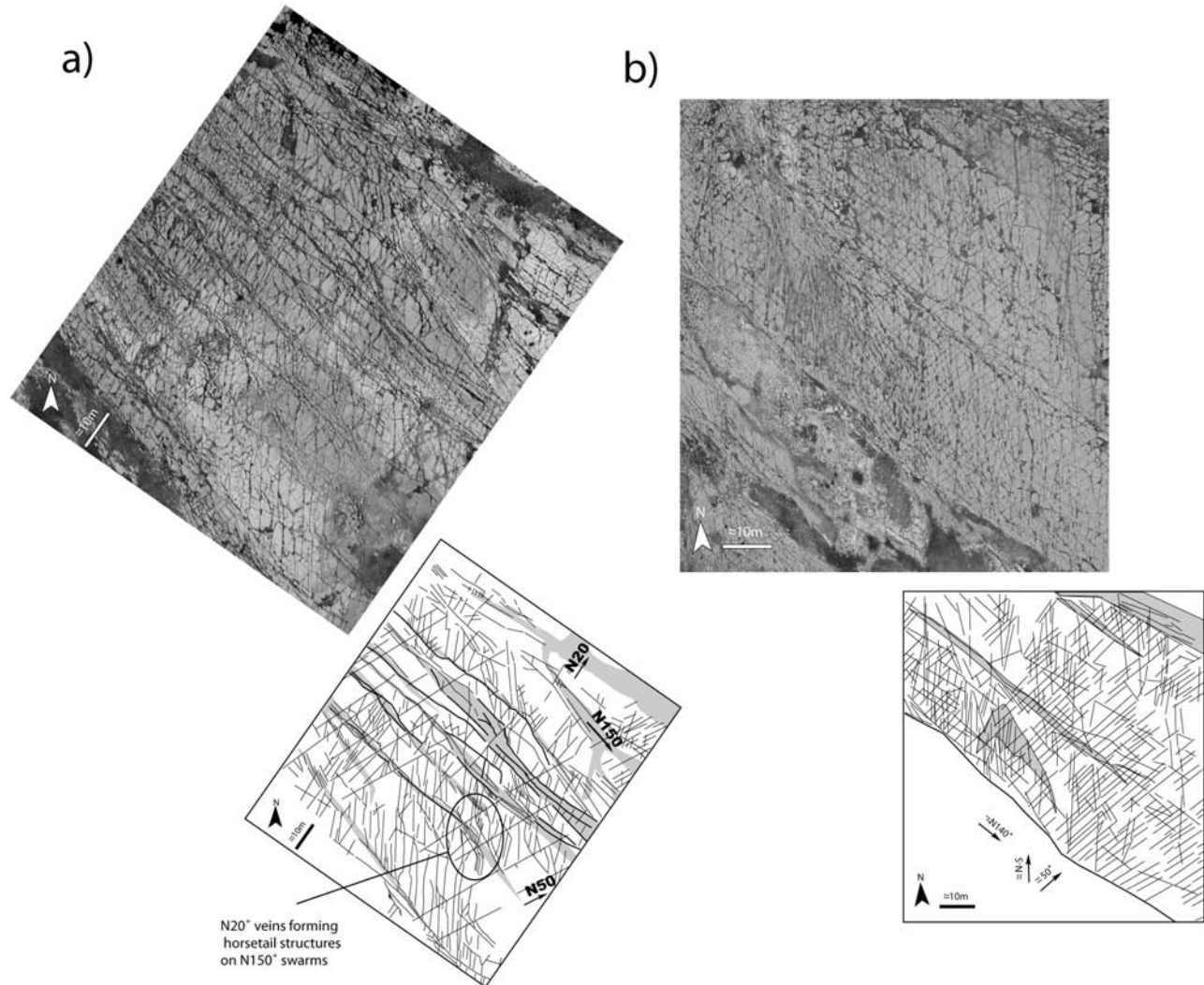
Figure 9. Main vein sets observed on the southern nose of the Asmari anticline (location on Figure 8b). (a) The regular vein set with an azimuth close to N50^\circ appears as the first set; N130^\circ trending veins form a series of clusters almost parallel to the fold axis; N20^\circ – 30^\circ and also N-S vein sets abut onto the previous sets. (b) Regular N50^\circ , N-S and N140^\circ – 150^\circ vein sets.
