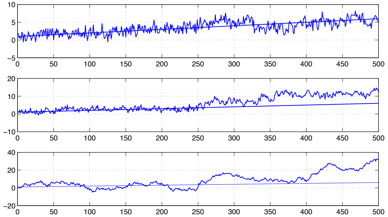
Figure 5: Comparison of trajectories simulated from the model (6.3) with a = 1 , b = .01 , change point \theta^* = 1/2 and different values of d_1 and d_2 : d_1 = .1 , d_2 = .4 (top); d_1 = .3 , d_2 = .6 (middle); d_1 = .8 , d_2 = 1.1 (bottom). The sample size is n = 500 .
