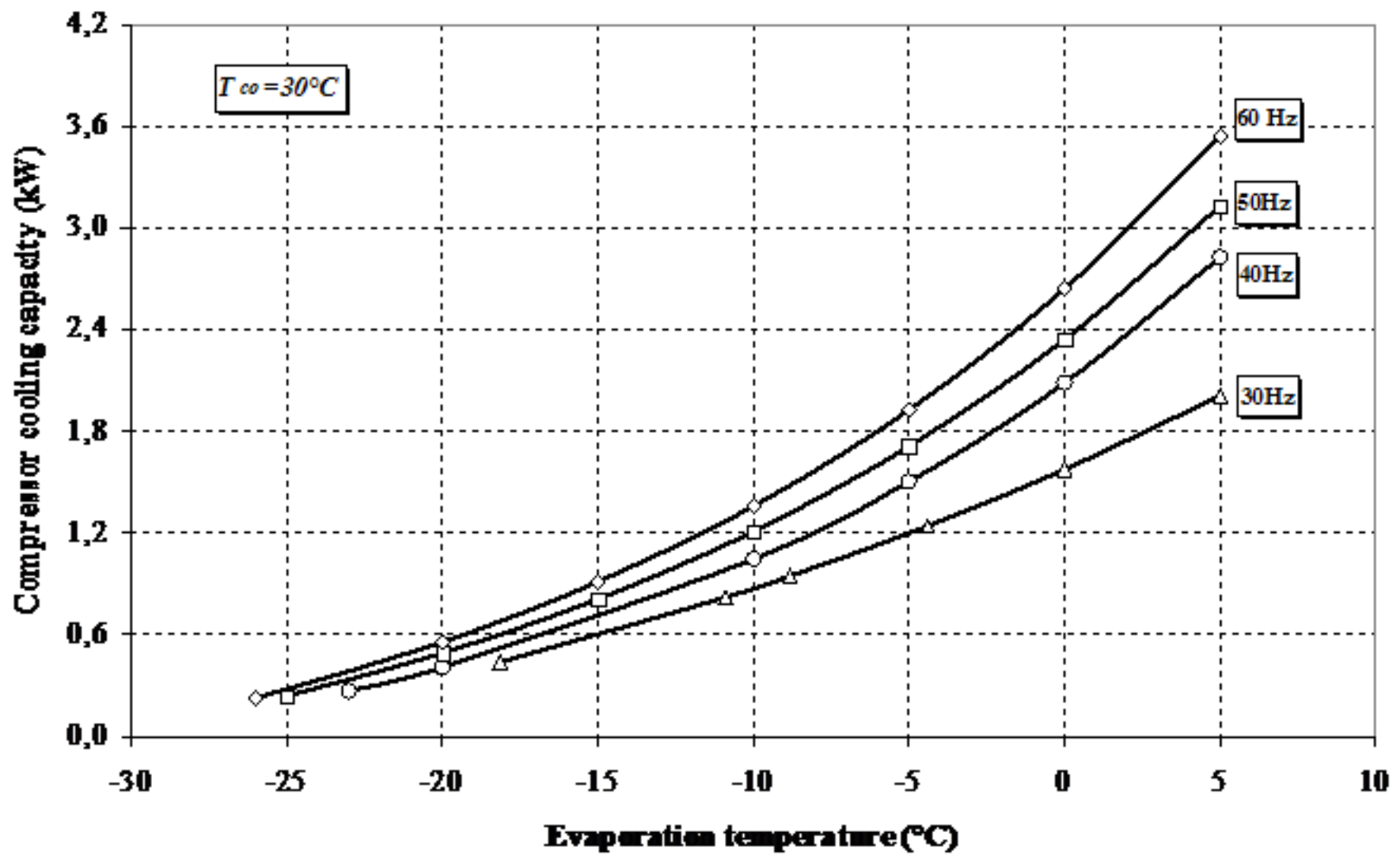
Figure 3. Cooling capacity when the compressor speed and evaporation temperature vary
