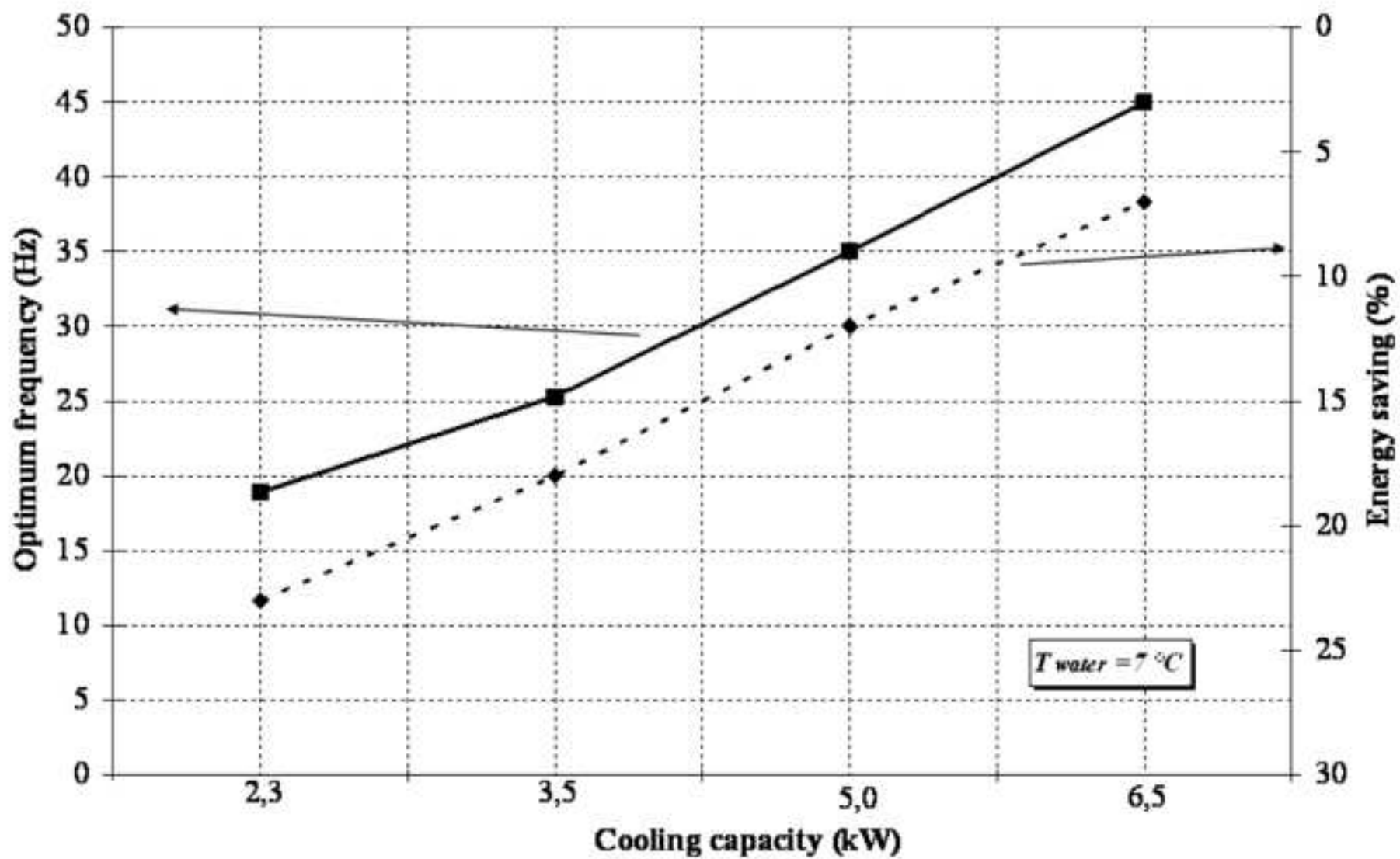
Figure 8. Energy saving corresponding to optimum frequency (water chiller)
