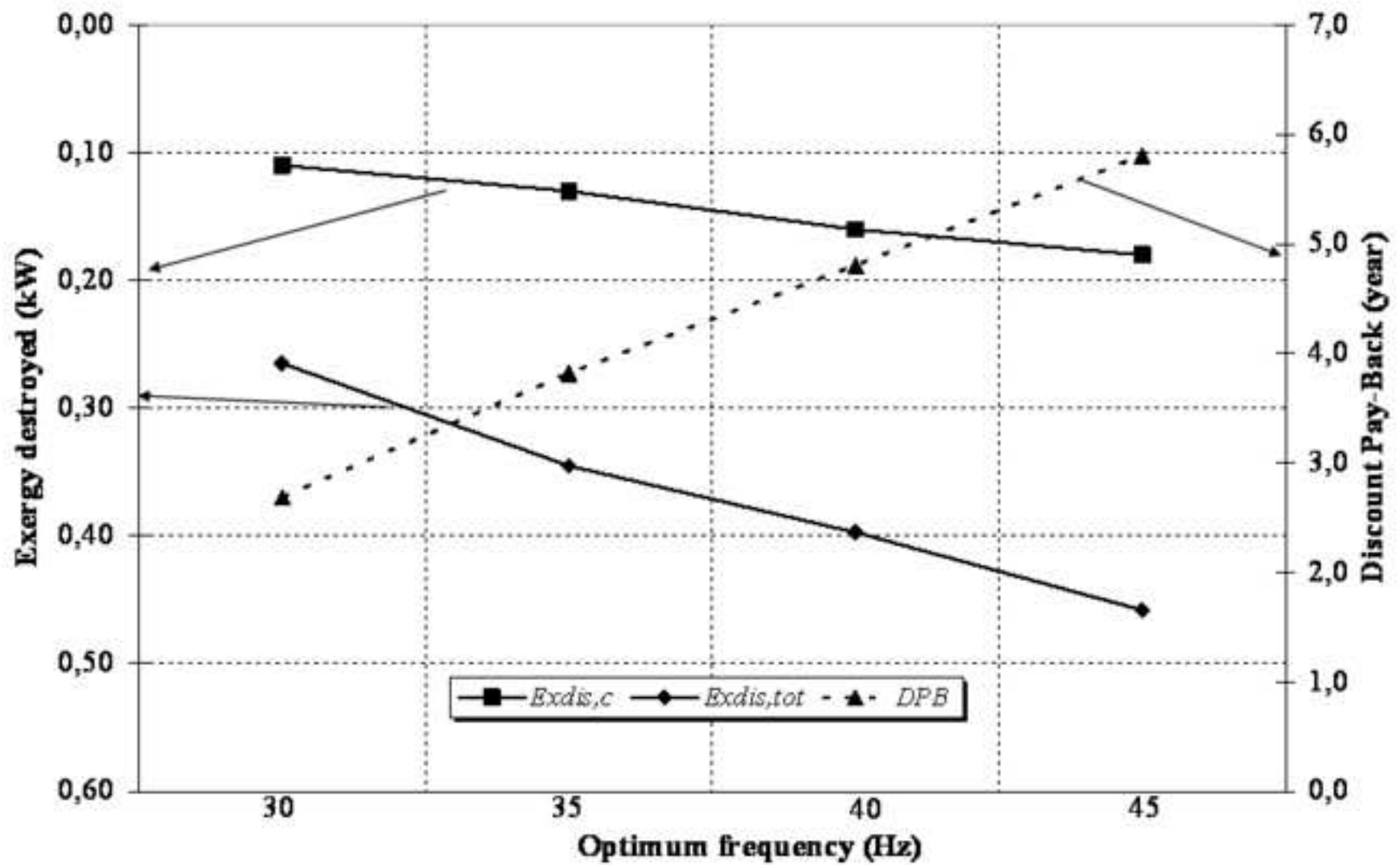
Figure 7. Exergy destruction rates and Discount Pay-Back referring to the reciprocating compressor
