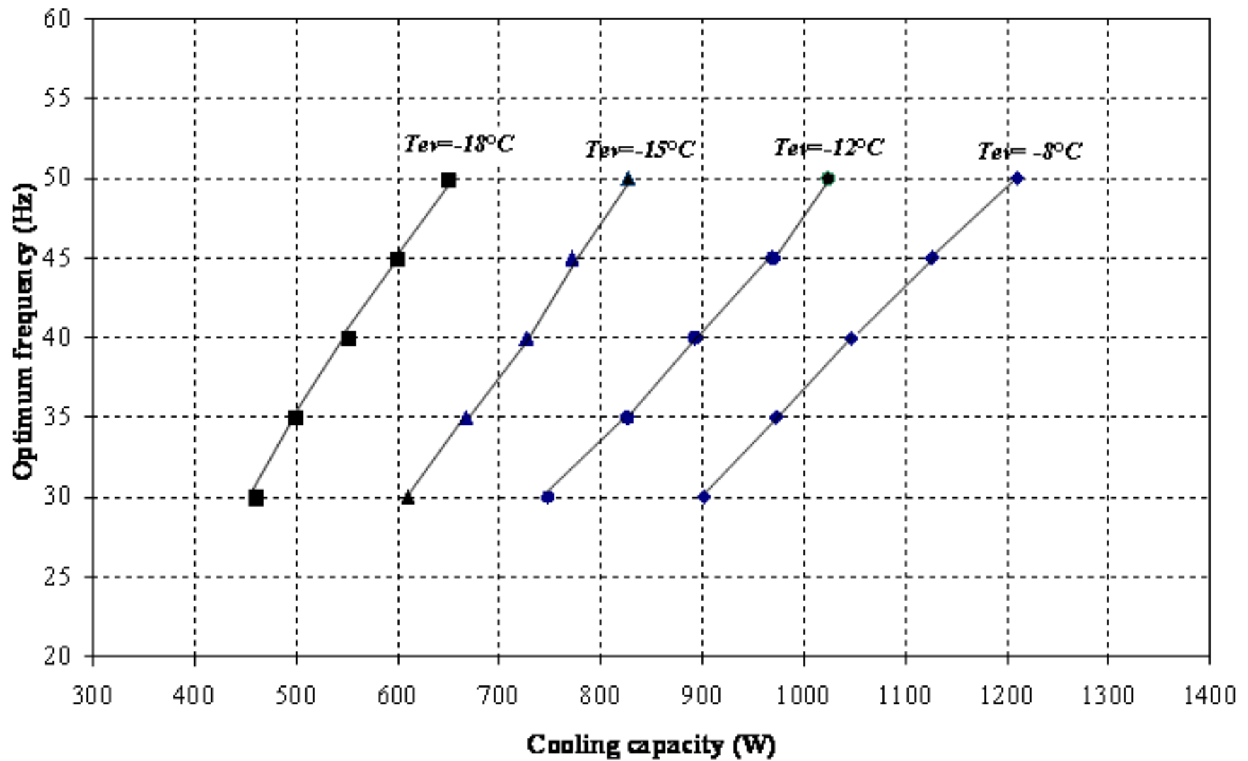
Figure 5. Optimum frequency referring to the reciprocating compressor for evaporation temperatures between -18^{\circ}C and -8^{\circ}C
