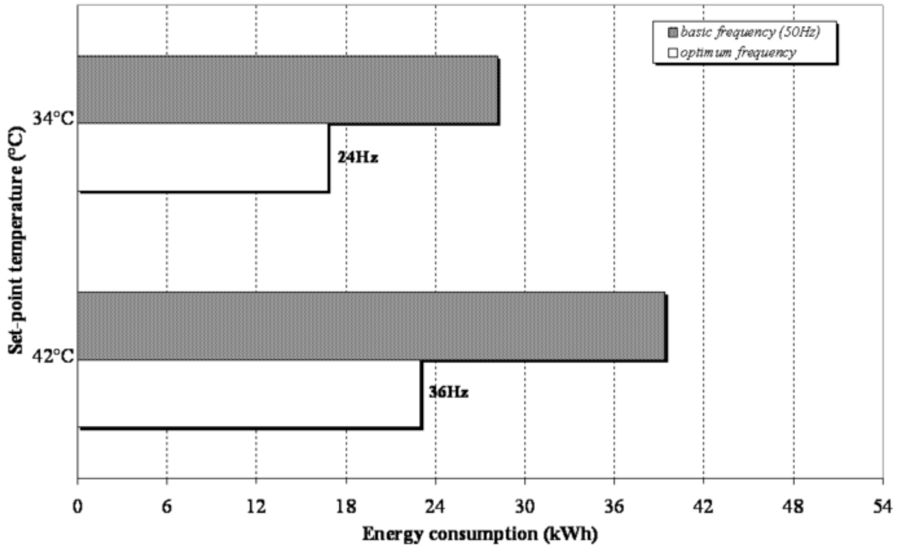
Figure 9. Energy saving corresponding to optimum frequency (heat pump)
