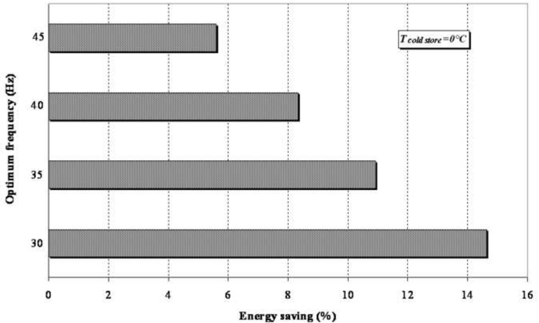
Figure 6. Energy saving corresponding to optimum frequency (reciprocating compressor)
