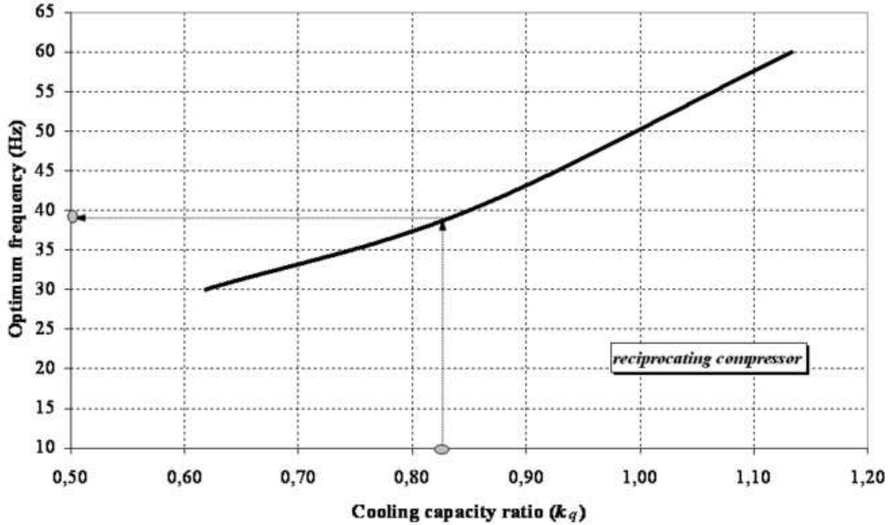
Figure 4. Optimum frequency determination referring to the reciprocating compressor under each working condition
