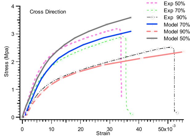
Figure 7. Modeling of the mechanical behavior of the corrugated cardboard under different rates of RH.
