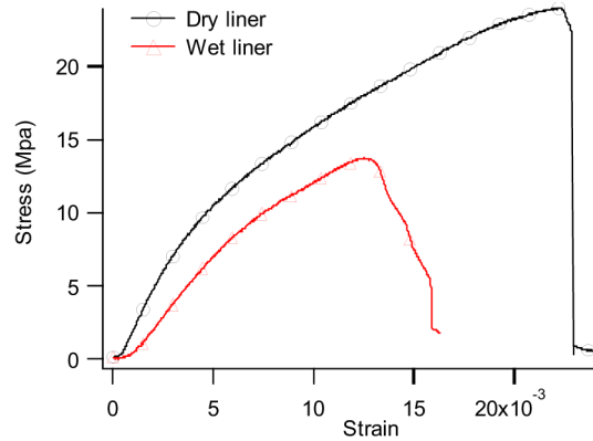
Figure 3. Tensile test of dry layer and wet one at 90% RH (CD).
