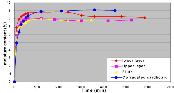
Figure 2. Moisture content at equilibrium for corrugated cardboard and its constituents.
