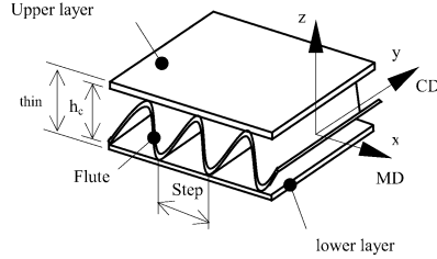
Figure 1. Cardboard panel geometry.
