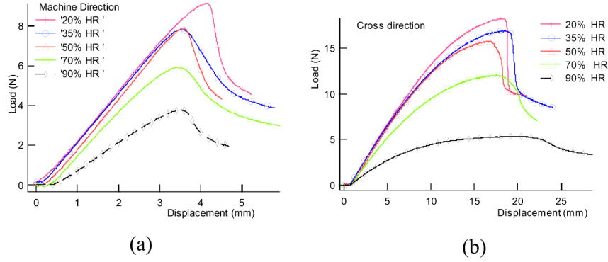
Figure 5. Three-point bending curves under different rates of RH.
