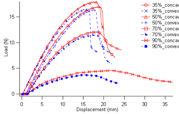
Figure 4. Bending test on convex and concave configuration under different rates of RH (corrugated cardboard in CD).
