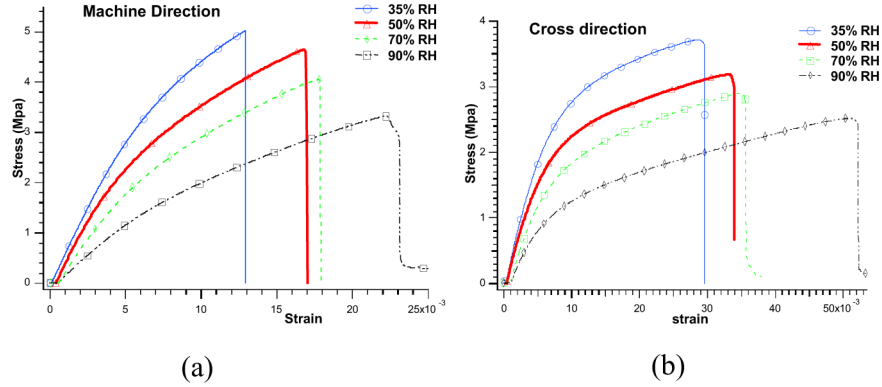
Figure 6. Tensile curves under different rates of RH.
