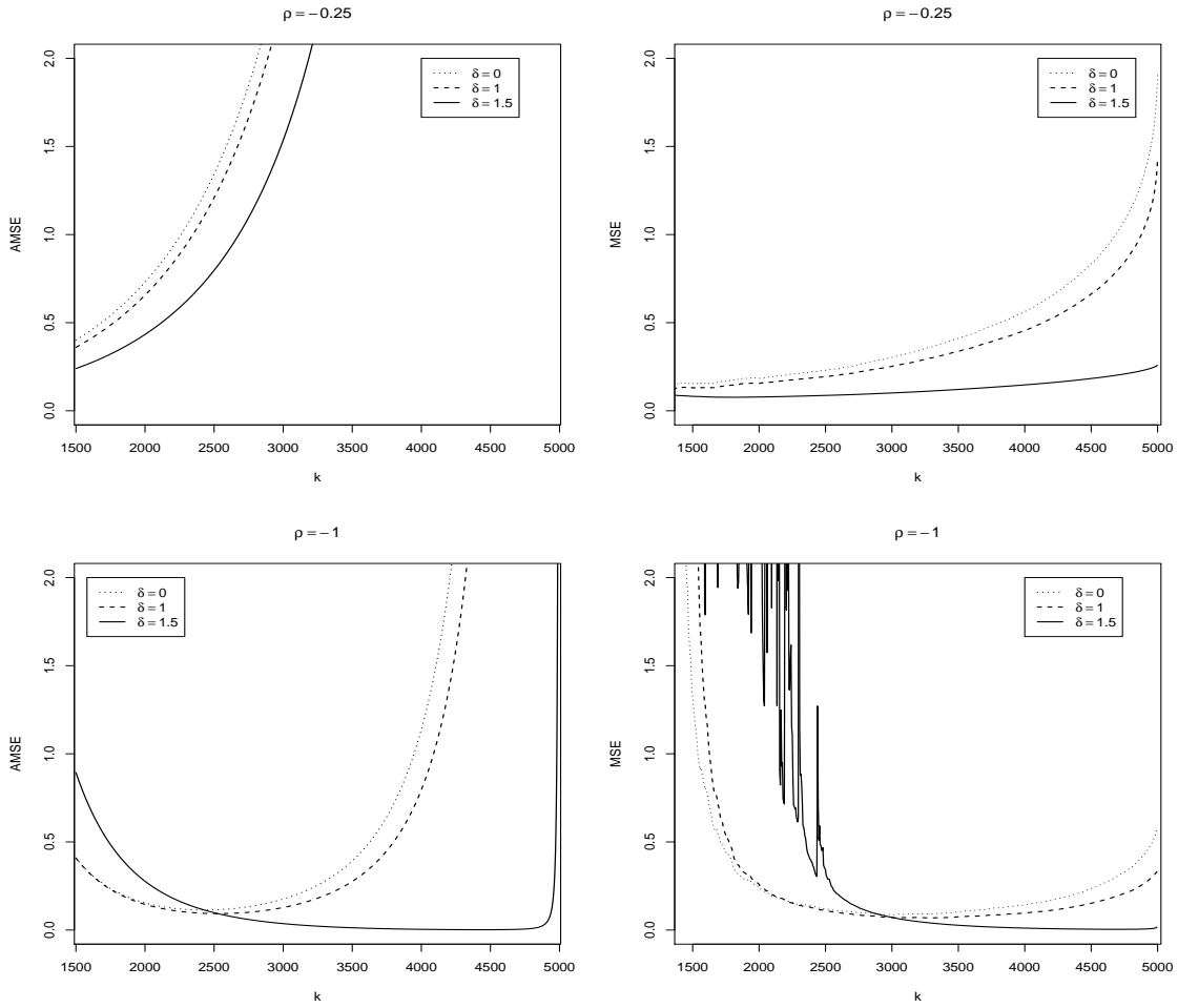
Figure 1: Asymptotic mean-squared errors (left) and empirical mean-squared errors (right) of \hat{\rho}_{n,0}^{(R)} , \hat{\rho}_{n,1}^{(R)} and \hat{\rho}_{n,2}^{(R)} as a function of k for a Burr distribution.
