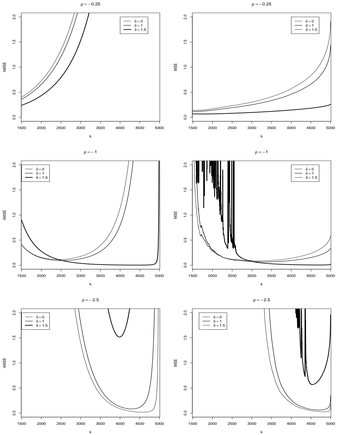
Figure 1: Asymptotic mean-squared errors (left) and empirical mean-squared errors (right) as a function of k for a Burr distribution.
