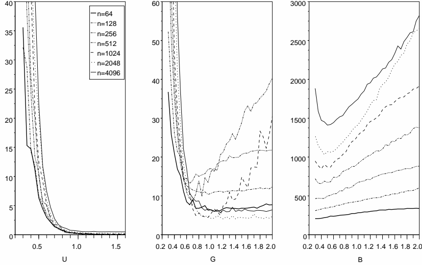
Figure 1: n \times \text{MISE}_n(\gamma) for (U) f = \mathbb{1}_{[0,1]} (the Haar basis is used) ; (G) f is the Gaussian density with mean 0.5 and standard deviation 0.25 (the Spline basis is used) ; (B) f is the renormalized Bumps signal (the Spline basis is used)
