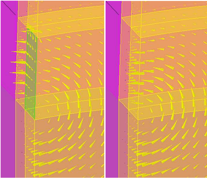
Fig. 11. Arrows of the current density in the tube, under the coil, for \omega t = 120^\circ : on the left, in the case « with a crack », on the right, in the case « without crack »
