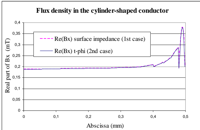
Fig. 7. Curves of the real part of the x component of flux density \mathbf{b} in the cylinder-shaped conductor, on the AB segment, at 100 kHz, in both cases
