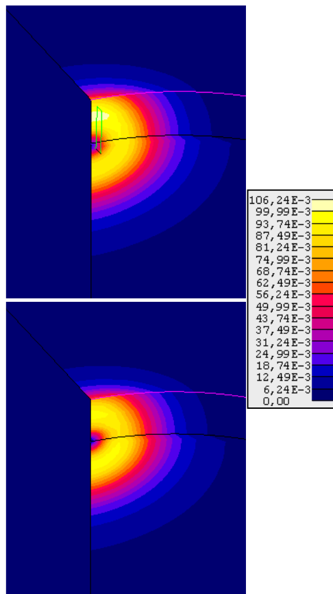
Fig. 14. Isovalues of the surface current density on the surface of the tube sheet, under the coil: at the top, in the case « with a crack », at the bottom, in the case « without crack ». The scale of surface current density is in A/m.
