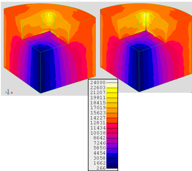
Fig. 5. Isovalues of the current density modulus in the cylinder-shaped conductor, at 100 kHz: on the left 1 st case (with parallelepiped conductor described with the surface impedance formulation), on the right 2 nd case (with parallelepiped conductor described with the \mathbf{t}\text{-}\phi formulation). The scale of the current density is in A/m 2 .
