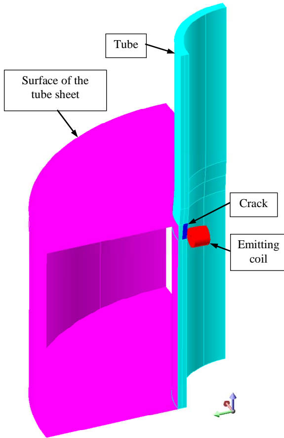
Fig. 9. Geometry described for the simulation.
