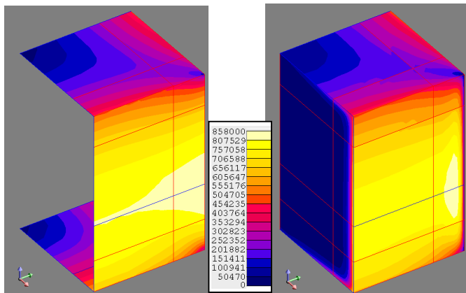
Fig. 4. Isovalues of the current density modulus in the parallelepiped conductor, at 100 kHz: on the left 1 st case (with parallelepiped conductor described with the surface impedance formulation), on the right 2 nd case (with parallelepiped conductor described with the \mathbf{t}\text{-}\phi formulation). The scale of the current density is in A/m 2 .
