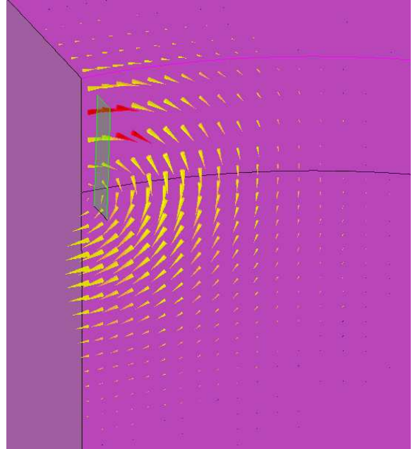
Fig. 13. Isovalues of the surface current density on the surface of the tube sheet, under the coil, in the case « with a crack », for \omega t = 90^\circ
