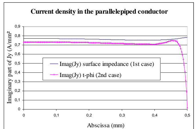
Fig. 6. Curves of the imaginary part of the y component of the current density \mathbf{j} in the parallelepiped conductor, on the AB segment, at 100 kHz, in both cases
