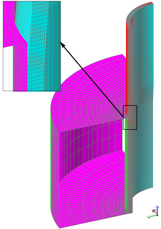
Fig. 10. Mesh of the tube and surface of the tube sheet, with a zoom of the cone-shaped zone of the tube.
