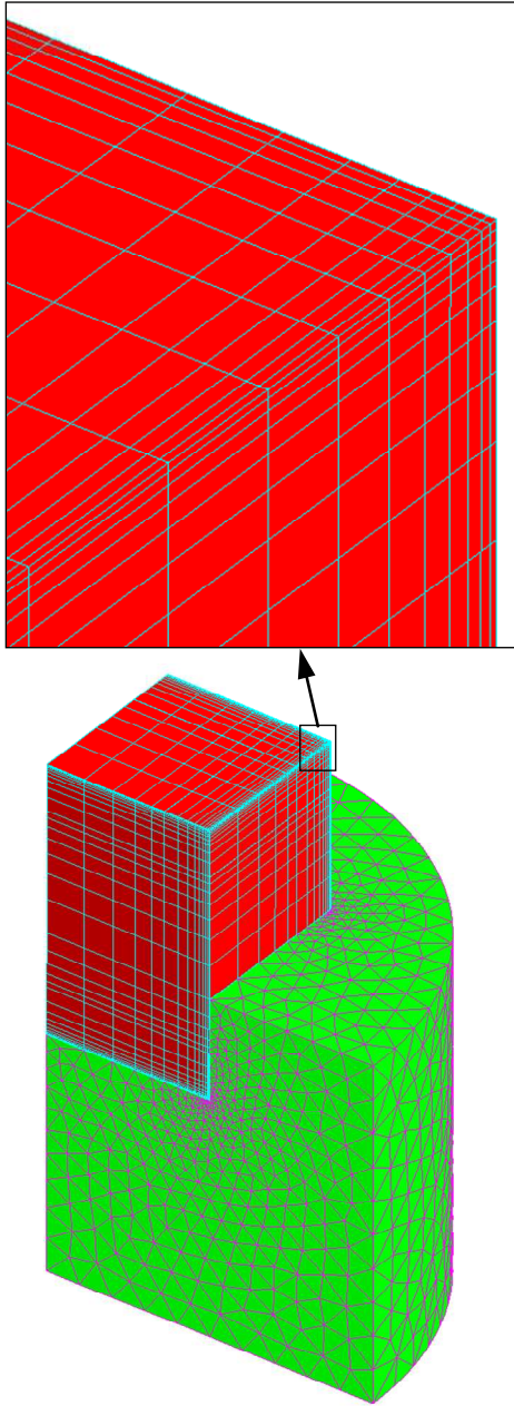
Fig. 3. Mesh of both conductors
