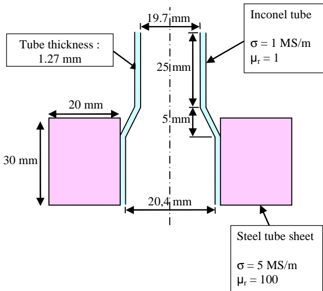
Fig. 8. Geometry of the tube and tube sheet, with material properties indicated.
