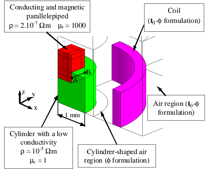
Fig. 2. Geometry description of the example. With the 3 symmetries, one eighth of the geometry is described
