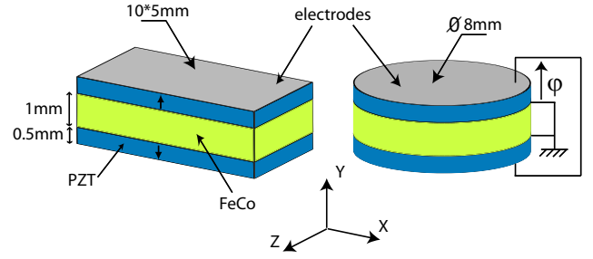
Fig. 2. FeCo/PZT multilayers for magnetolectric sensors.
