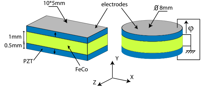
Fig. 2. FeCo/PZT multilayers for magnetoelectric sensors.
