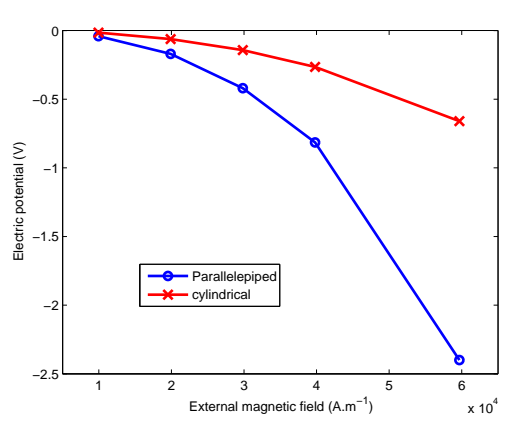
Fig. 13. Electric potentials versus external magnetic field.
