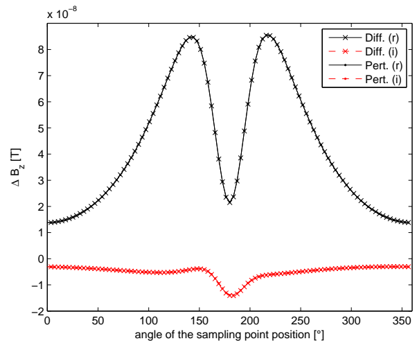
Fig. 8. Variation due to the flaw on the longitudinal ( z ) component. (pert.) denote the value obtained with perturbation, while (diff.) the value obtained with difference between the perturbed and unperturbed solutions. (r) denotes the real part, (i) the imaginary part.
