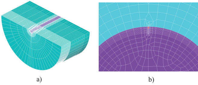
Fig. 2. a) One fourth of the hexahedral mesh used in the NDT application. b) A zoom on the mesh in the neighborhood of the flaw.
