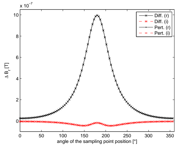
Fig. 7. Variation due to the flaw on the radial component. (pert.) denote the value obtained with perturbation, while (diff.) the value obtained with difference between the perturbed and unperturbed solutions. (r) denotes the real part, (i) the imaginary part.
