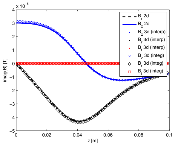
Fig. 5. The computed imaginary part of the induction magnetic field B along a sampling line in the case of unperturbed problem, compared with an axisymmetrical two-dimensional FEM simulation. B is found both with direct interpolation (interp) and using the Biot-Savart law (integ).
