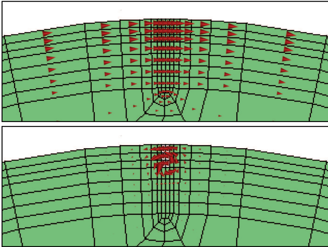
Fig. 9. On the top, the current density in the neighborhood of the flaw obtained using the unperturbed configuration. On the bottom, the current density obtained with the perturbation problem, which is confined in the neighborhood of the flaw.
