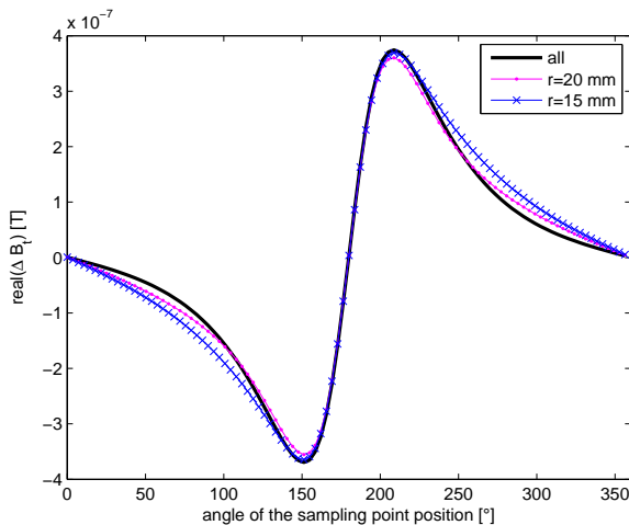
Fig. 10. The real part of the tangential component of the magnetic induction due to the flaw obtained with the reduced meshes is compared to the one obtained with the original mesh.
