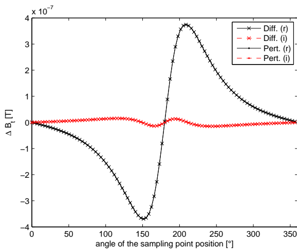
Fig. 6. Variation due to the flaw on the tangential component. (pert.) denote the value obtained with perturbation, while (diff.) the value obtained with difference between the perturbed and unperturbed solutions. (r) denotes the real part, (i) the imaginary part.
