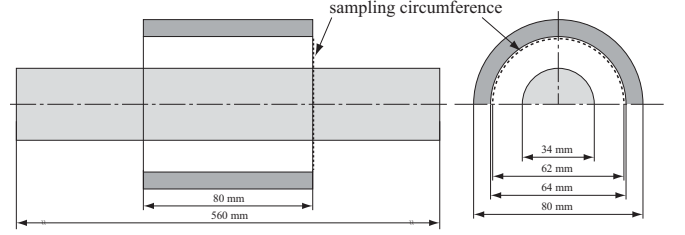
Fig. 1. The geometry of the eddy-currents problem.
