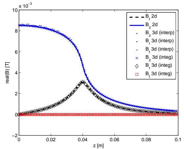
Fig. 4. The computed real part of the induction magnetic field \mathbf{B} along a sampling line in the case of unperturbed problem, compared with an axisymmetrical two-dimensional FEM simulation. \mathbf{B} is found both with direct interpolation (interp) and using the Biot-Savart law (integ).
