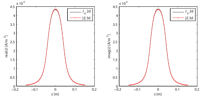
Fig. 3. The computed current density \mathbf{J} (real part on the left, imaginary part on the right) along a sampling line in the case of unperturbed problem, compared with an axisymmetrical two-dimensional FEM simulation.
