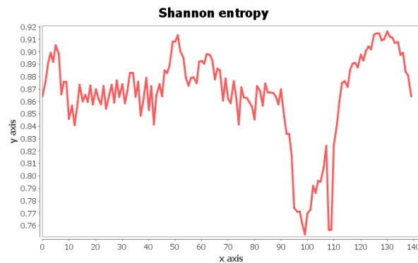
Figure 10. Profile of the polyline presented in the Fig. 4 (using the Shannon entropy measure).
