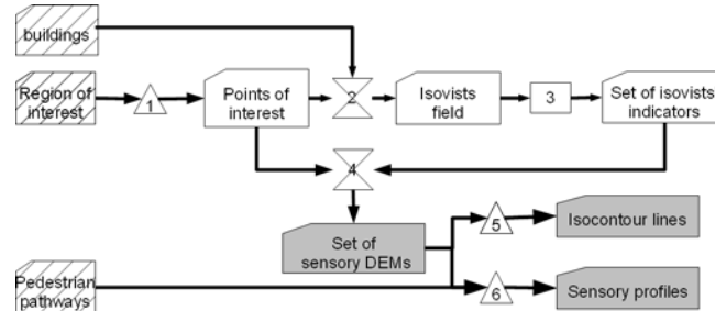
Figure 2. The geo-processing schema we have adopted. Input maps are 45 degrees wide hatched, intermediate results have no background colour and final output results are grey coloured
