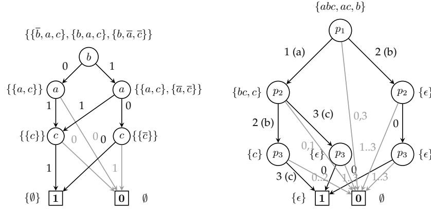
Figure 4.2: Different representations of scenarios abc , ac and b by means of DDs. On the left hand side, scenarios are considered as cuts (note that in this case, \bar{b} and \bar{a}\bar{c} are implicit in ac and b ). Each variable of the DD corresponds to an event and are ordered as b < a < c . Edges to leaf node 0 are drawn in gray. On the right hand side, scenarios are viewed as sequences where a = 1 , b = 2 and c = 3 (recall observer described in chapter 2). Length of sequences is bound by k = 3 . Note that for sequences with less than k events, scenarios are padded with 0s.
