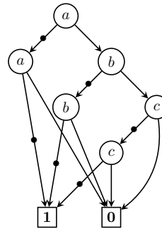
Figure 3.4: A RLDD for Sqr(\{a, b, c\}) .
