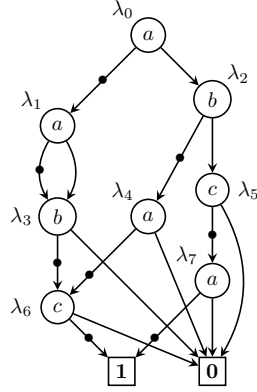
Figure 3.2: RLDD encoding the same language that the RLDD on figure 3.1. The order a < b < c is used.
