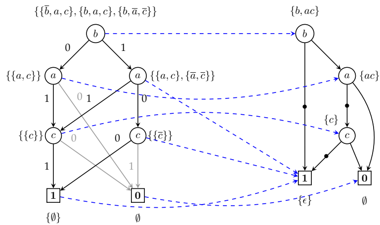
Figure 4.4: Application of the dd-to-min-r1dd algorithm onto the DD encoding cuts abc , ac and b depicted on figure 4.2. Dashed arrows show the mapping realized by the algorithm between DD (on the left) and RLDD nodes (on the right). Variables are ordered as follows: b < a < c .
