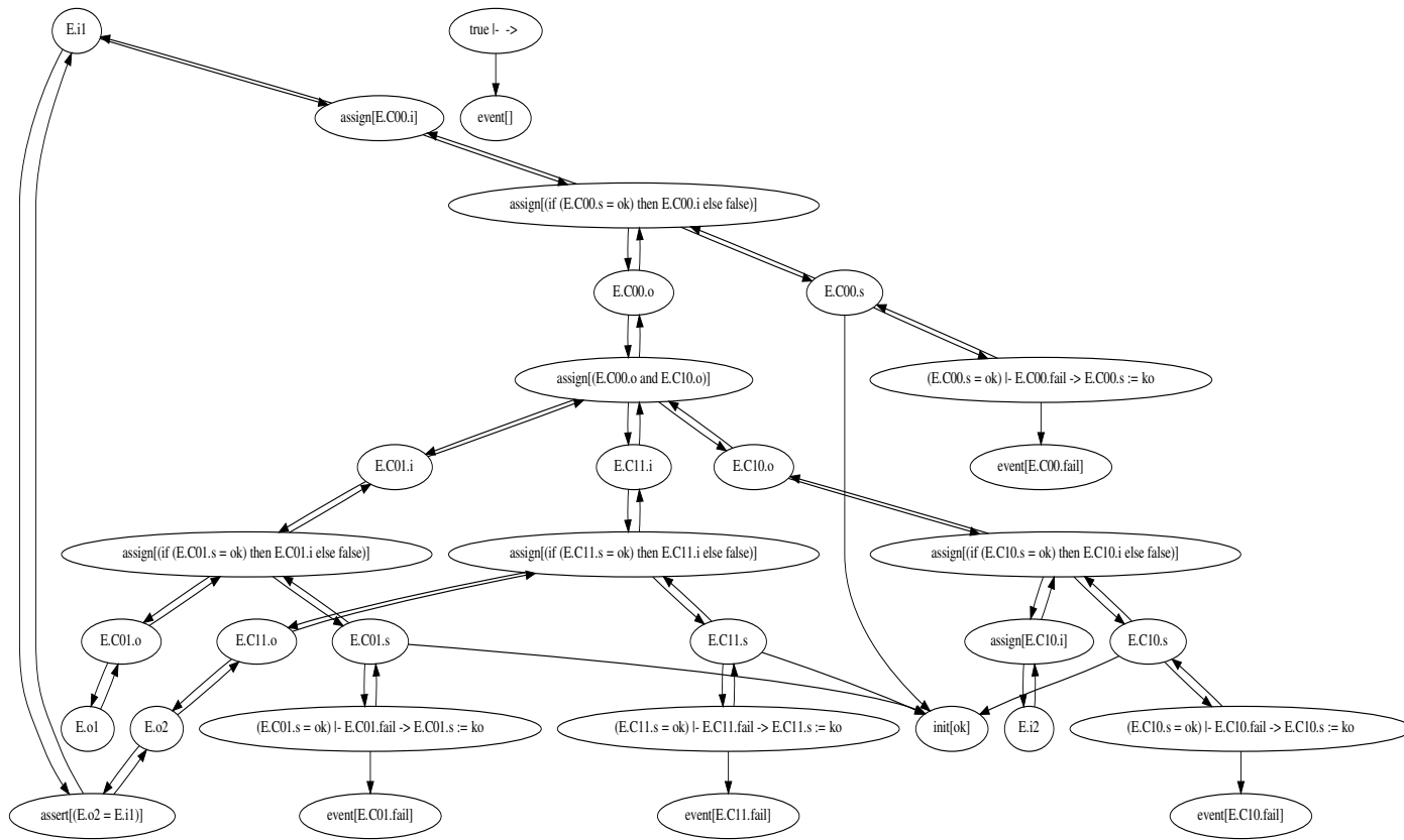
Figure 5.7: Dependency graph of the system with a loop.
