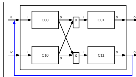
Figure 5.4: A feedback loop is added that wires up output o2 to input i1
