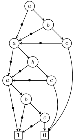
Figure 3.3: A RLDD encoding for \{a, b, c\}^3
