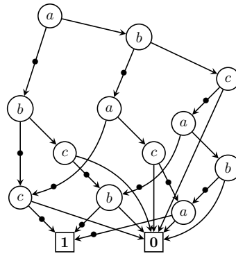
Figure 3.5: A RLDD encoding U_3 = \{a, b, c\}^3 \div Sqr(\{a, b, c\})
