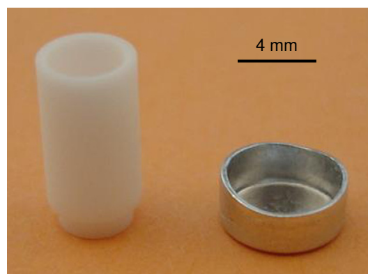
Fig. 11. DTA (left) and DSC (right) crucibles.
