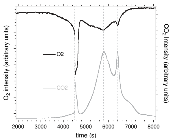
Fig. 5. Mass Spectroscopy Analysis of \text{O}_2 and \text{CO}_2 obtained at 5\text{ }^{\circ}\text{Cmin}^{-1} up to 500\text{ }^{\circ}\text{C} under dry air (3 l/h).
