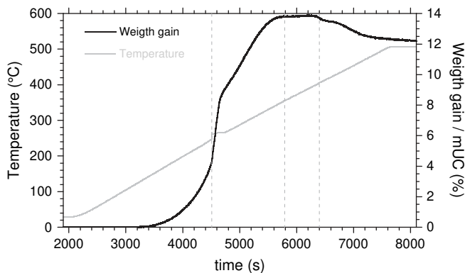
Fig. 4. Thermogravimetric Analysis obtained at 5\text{ }^{\circ}\text{Cmin}^{-1} up to 500\text{ }^{\circ}\text{C} under dry air (3 l/h).
