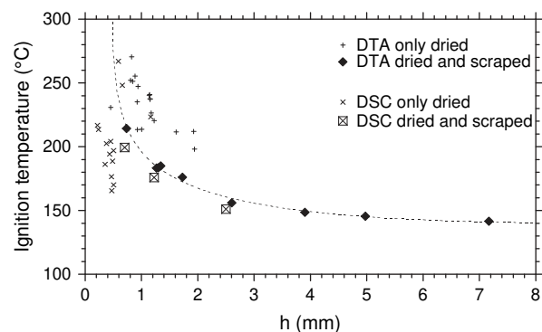
Fig. 14. Ignition temperature vs powder bed height in DTA crucibles and DSC crucibles. DTA ◆ and DSC ⊠: UC powder dried and scraped (the powder bed height is well controlled). DTA + and DSC ×: UC powder only dried in the crucibles (the powder height is calculated from UC mass and do not take into account the powder sample shape).
