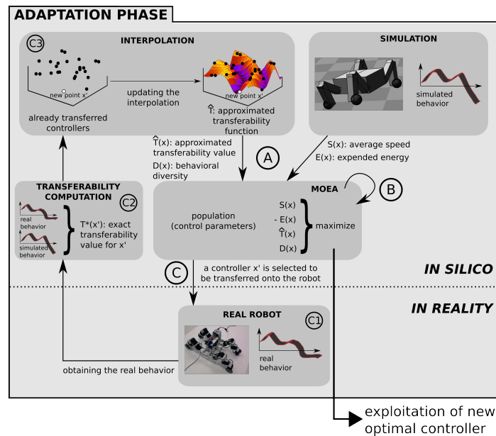
Fig. 3. Outline of the adaptation phase. The four objectives are computed for the controllers (step A), which are optimized during N generations with a multi-objective evolutionary algorithm (MOEA, step B). The controller with the highest behavioral diversity is then transferred onto the real robot and the generated data allows to update the approximated transferability function (steps C1 to C3).
