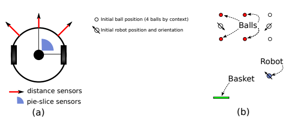
Figure 3: (a) Overview of the simulated mobile robot for the ball-collecting task. The robot is equipped with two pie-slice sensors that detect the balls and two more that detect the basket. The view range of the right sensors is depicted on the figure, the left ones are symmetric. The robot is moved by two motors, the neural network setting the speed of each of them. (b) Map employed in this set of experiments. Several initial positions and orientations of the robot are depicted with a circle and an arrow.
