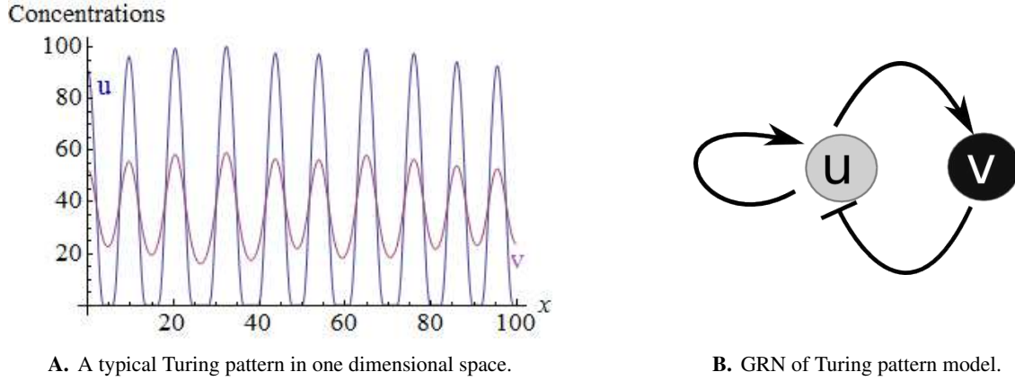
Figure 5. A Turing pattern and the corresponding GRN.
