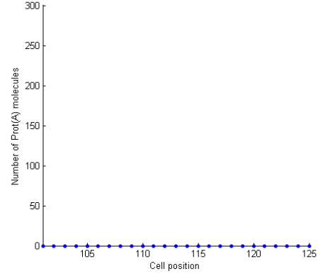
B. Prot(A): N_a = 25 , N_p = 100 , t = 6 \times 10^5
