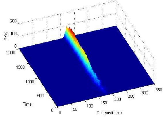
B. Initial distribution of u is localized at cell 175.
