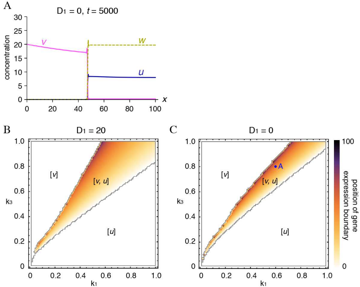
Figure 11. Simulations of the PDE model show that cell-to-cell communication by the diffusible factor w is dispensable for pattern formation, but is essential for community effects. (A) Steady state profile. (B, C) Phase diagrams in the parameter plane ( k_1, k_3 ) with D_1 = 20 (B) and D_1 = 0 (C). The position of the expression boundary for [v, u] pattern is colour-coded as indicated. Borders between the patterns [u] , [v] and [v, u] are indicated by grey lines. Simulation parameters for (B,C) are listed in Table 5, except k_1, k_3 and D_1 as indicated in the panels.
