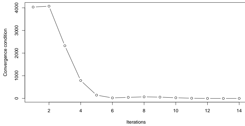
Figure 4.2: Evolution of the log-likelihood (top) and of the convergence criterion \delta^{(q)} (bottom) according to the iterations of the Fisher-EM algorithm on the Iris dataset.
