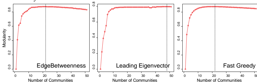
Fig. 1. Modularity values obtained for three hierarchical algorithms when applied to our data. Only the higher levels of the hierarchy are represented. The dotted lines indicate the partitions of maximal modularity.
