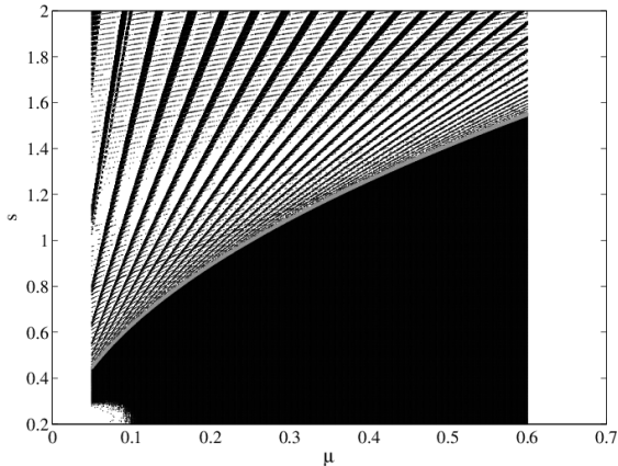
Figure 3. Numerical basin of attraction of the Petviashvili scheme in the phase space (s, \mu) for \varepsilon = 0.15 . Solitary waves (localized traveling waves) occur below the gray boundary curve \Gamma , which separates the region of periodic waves.
