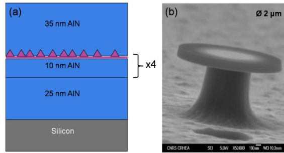
Figure 1 a) Epitaxial structure : the optically active area above the Silicon substrate contains 4 periods of GaN/AlN QDs layers. b) Scanning Electron Microscopy image of a 2 μm in diameter microdisk.
