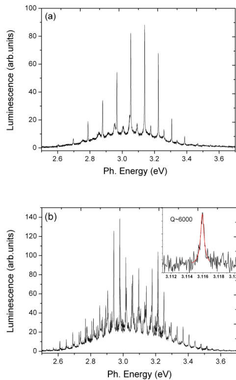
Figure 2 Photoluminescence spectra of a (a) 2 μm and (b) 5 μm in diameter microdisk. Inset : High resolution spectrum of a WGM of high Q value, i.e. Q \sim 6000 ; the peak is fitted by a Lorentzian line shape (red line).
