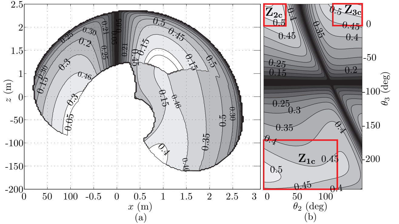
Figure 3: Contours of the inverse condition number of \mathbf{J}_N : (a) in the robot Cartesian workspace and (b) in the joint space (\theta_2, \theta_3)
